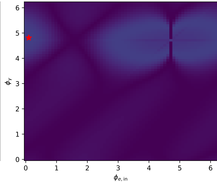
high_s_high_theta_in_high_Egamma min D_W=0.9428
