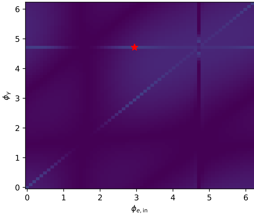
high_s_high_theta_in_low_Egamma min D_W=0.9429
