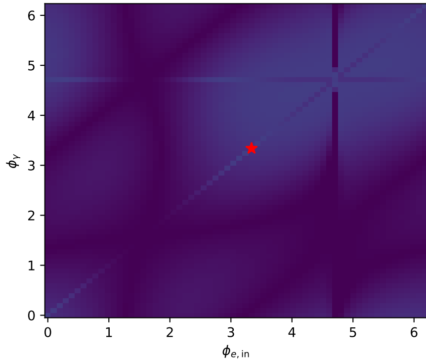
high_s_high_theta_in_mid_Egamma min D_W=0.9428
