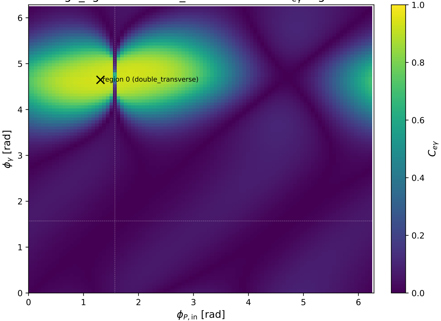
high_Egamma double_transverse: max C_{e\gamma} regions
