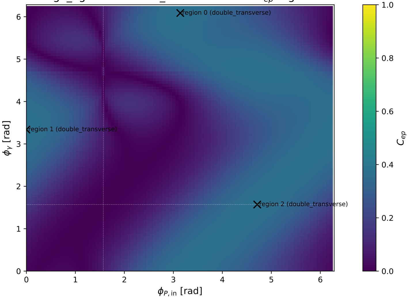
high_Egamma double_transverse: max C_{ep} regions
