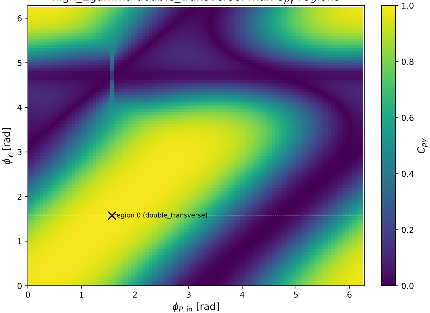
high_Egamma double_transverse: max C_{p\gamma} regions
