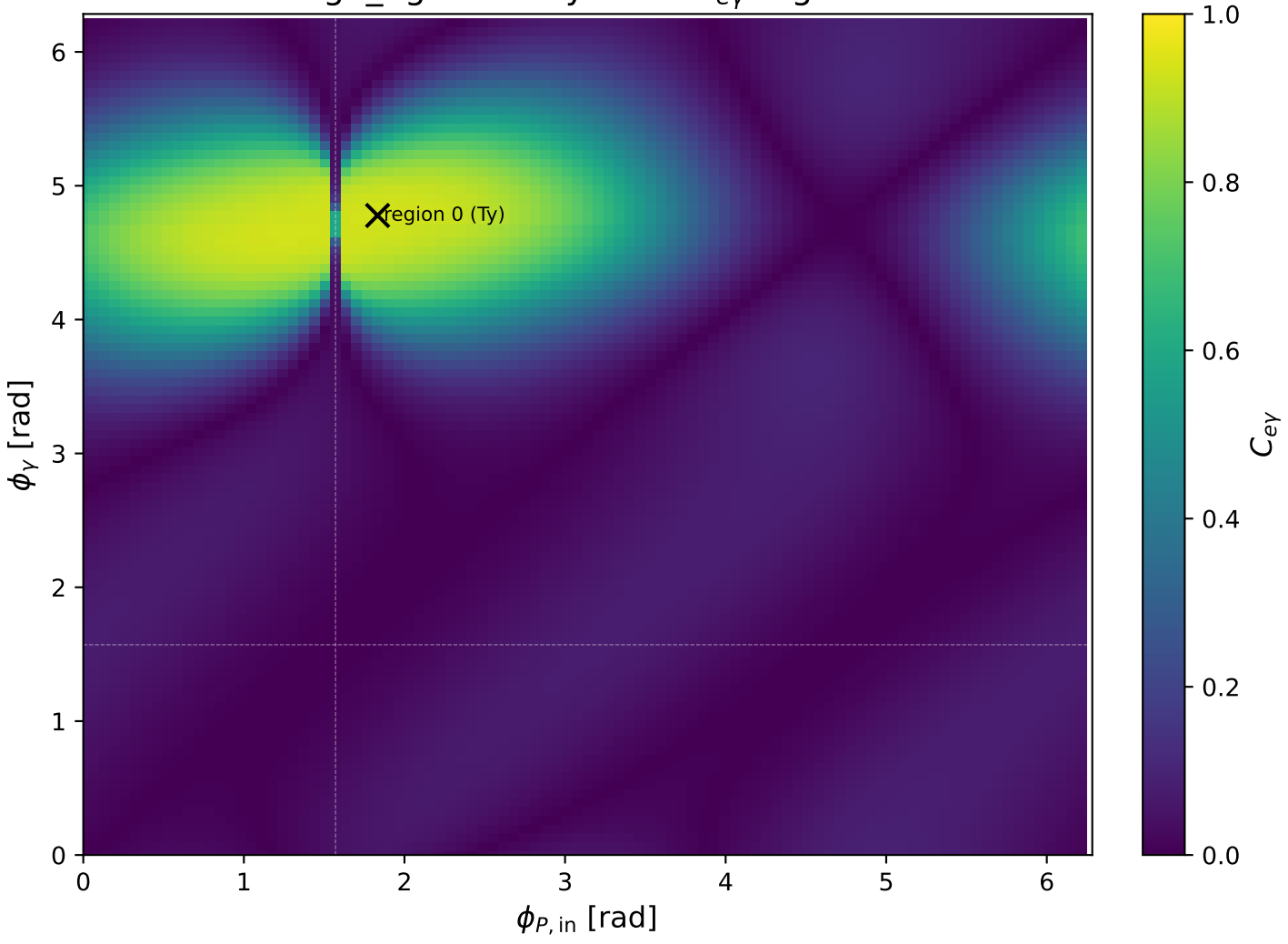
high_Egamma Ty: max C_{e\gamma} regions
