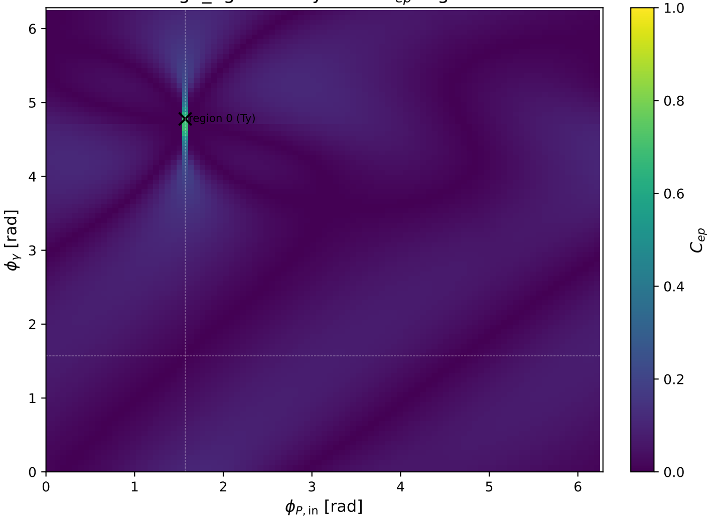
high_Egamma Ty: max C_{ep} regions
