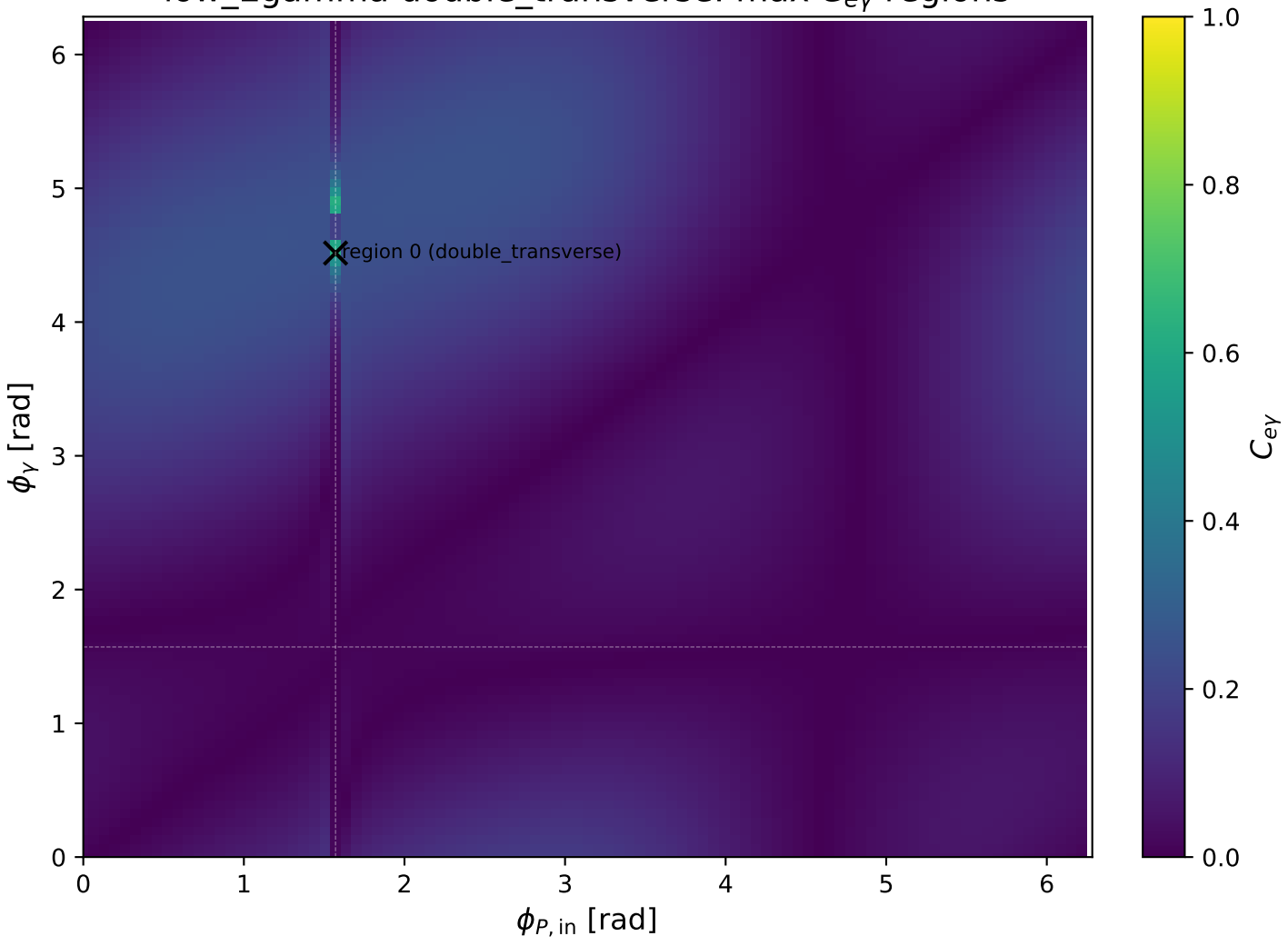
low_Egamma double_transverse: max C_{e\gamma} regions
