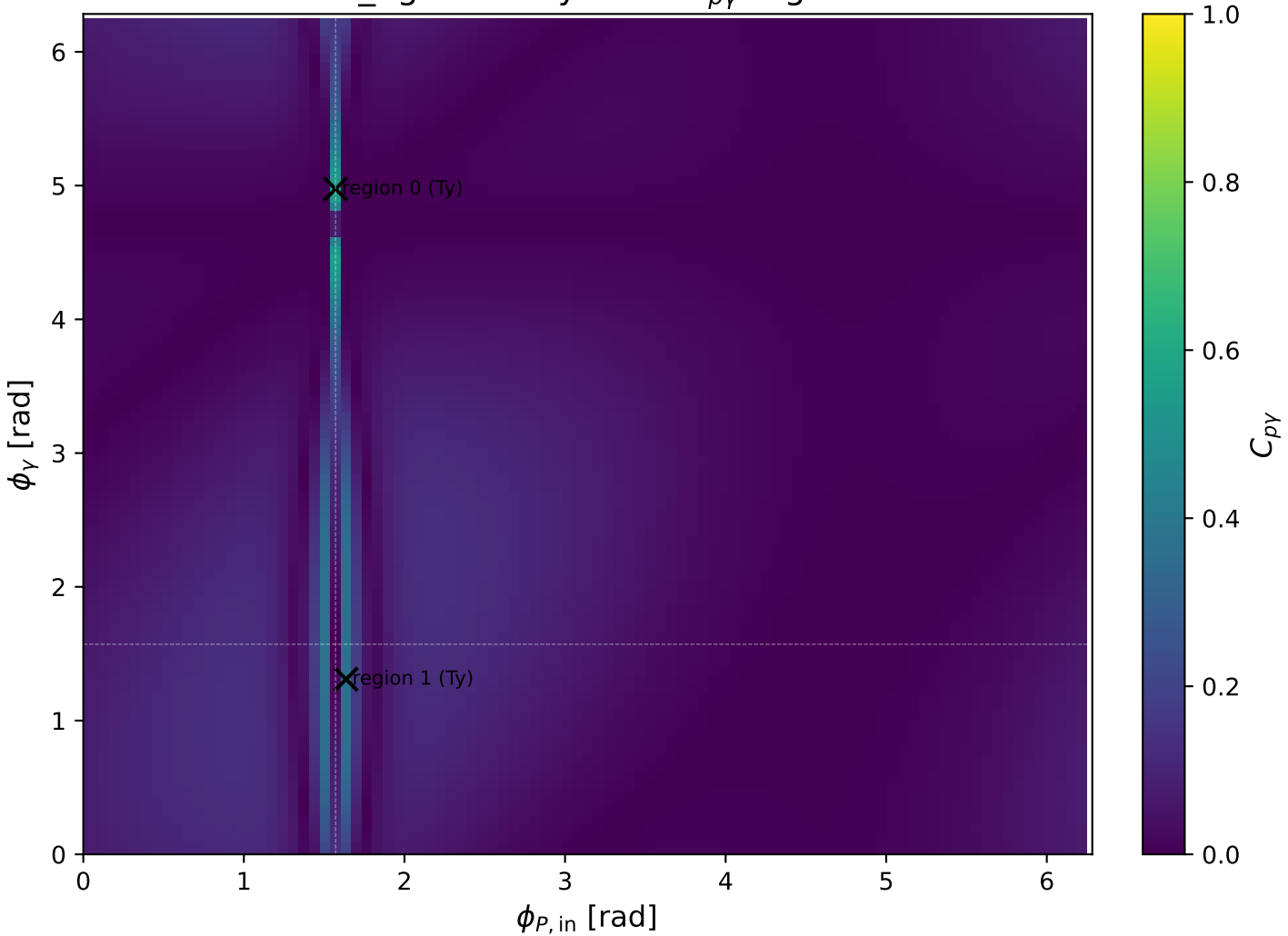
low_Egamma Ty: max C_{p\gamma} regions
