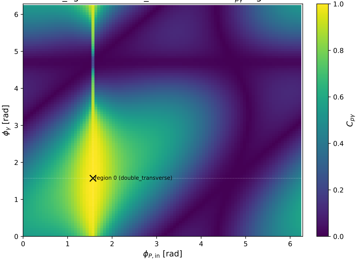
mid_Egamma double_transverse: max C_{p\gamma} regions
