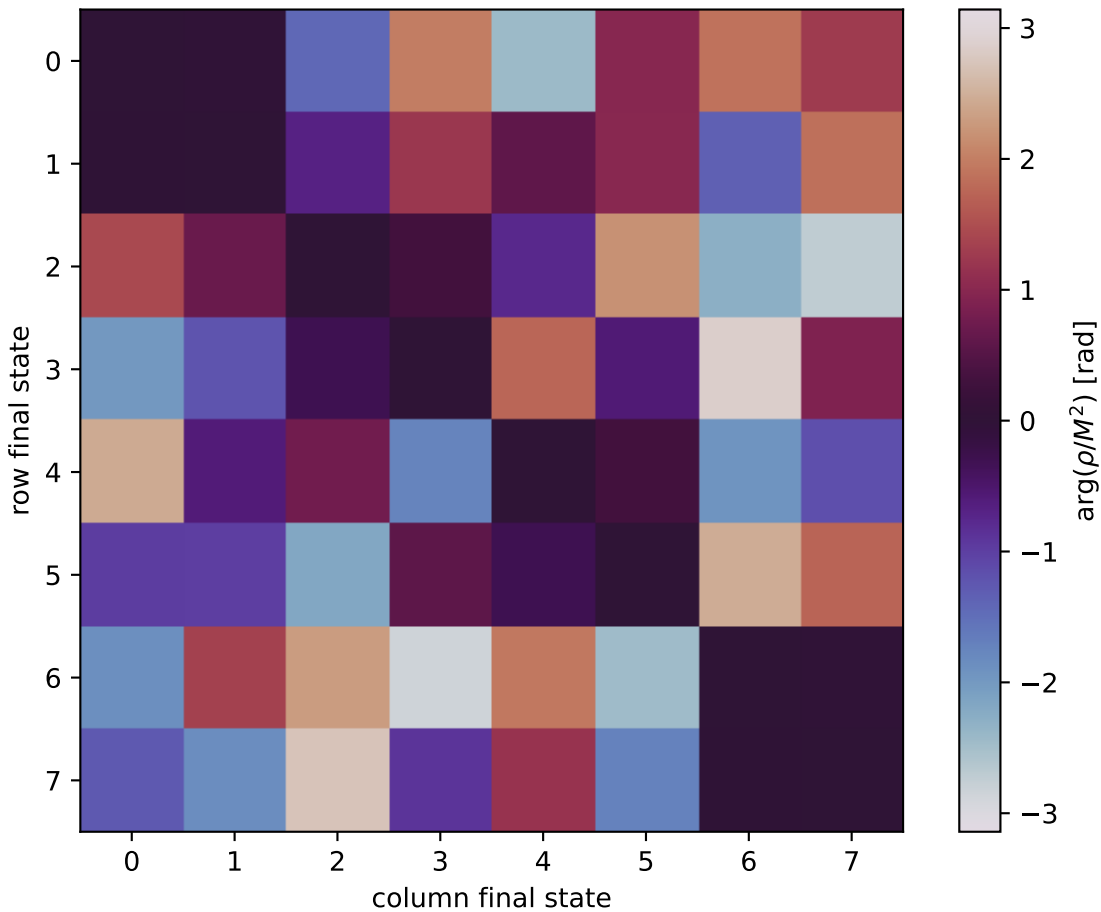
\arg(\rho/M^2) at Q2=1, t=-0.35
