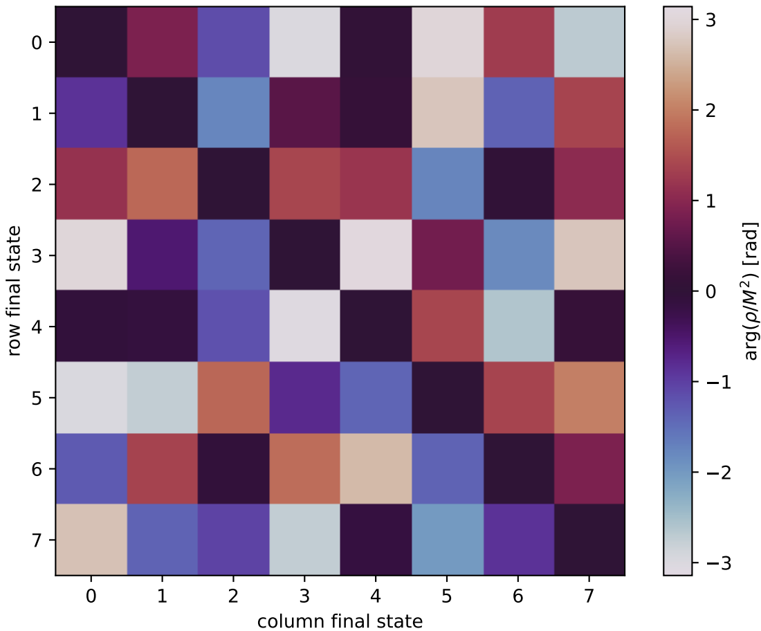
\arg(\rho/M^2) at Q2=3, t=-0.35
