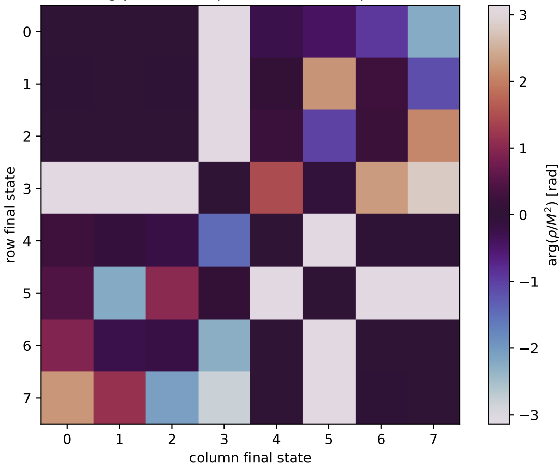
\arg(\rho/M^2) at unpolarized, Q2=2, phi=0
