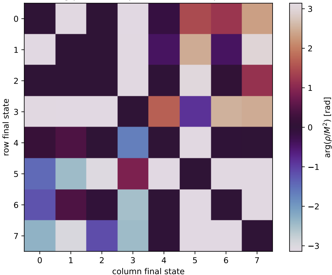
\arg(\rho/M^2) at unpolarized, Q2=4, phi=0
