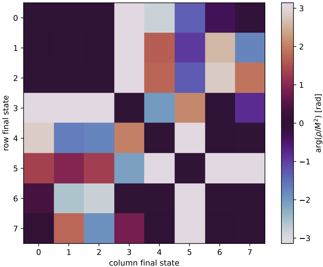
\arg(\rho/M^2) at unpolarized, Q2=5, phi=0
