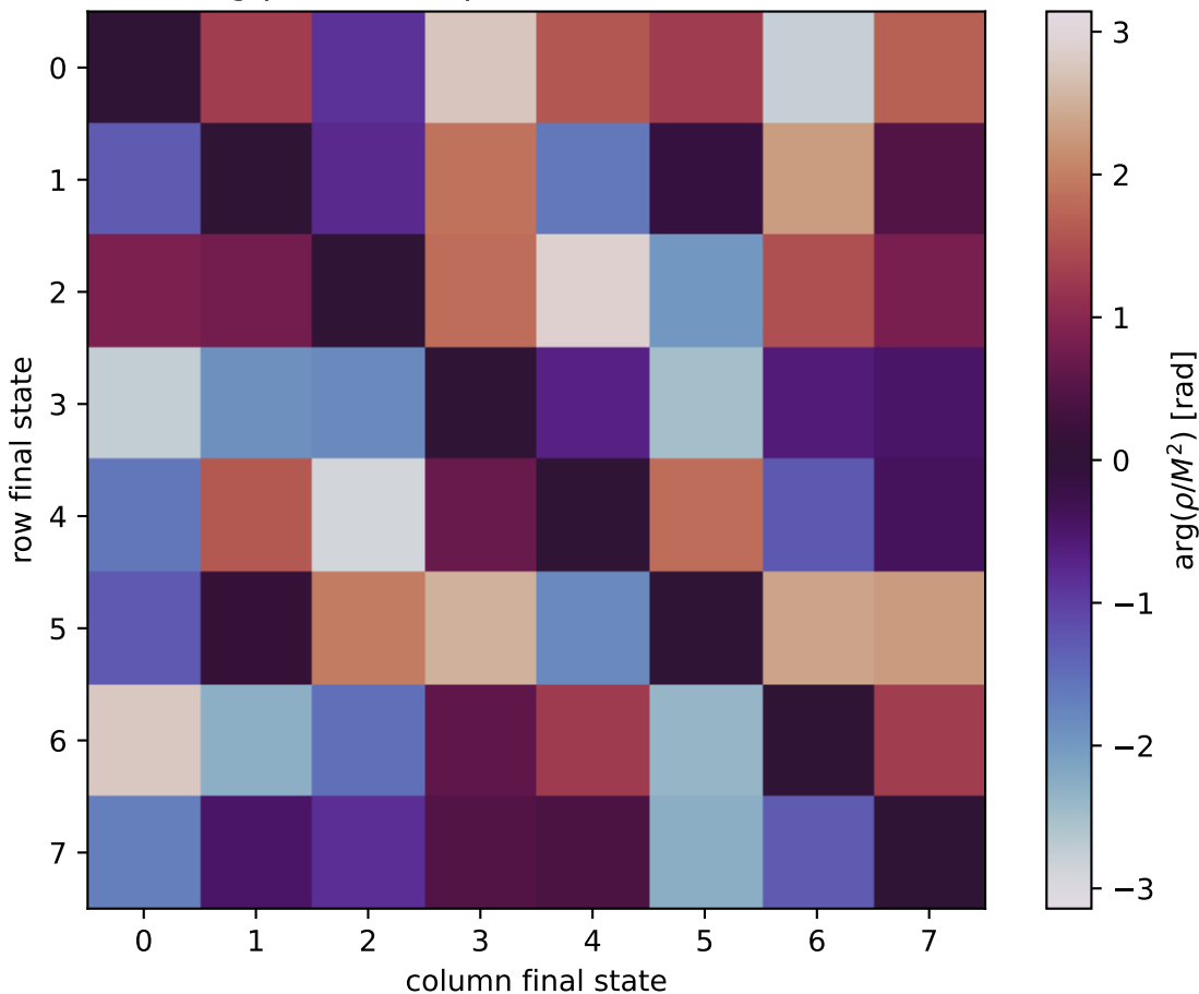
\arg(\rho/M^2) at unpolarized, Q^2=3 , t=-0.8
