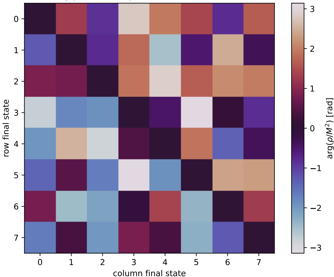
\arg(\rho/M^2) at unpolarized, Q2=4, t=-0.7
