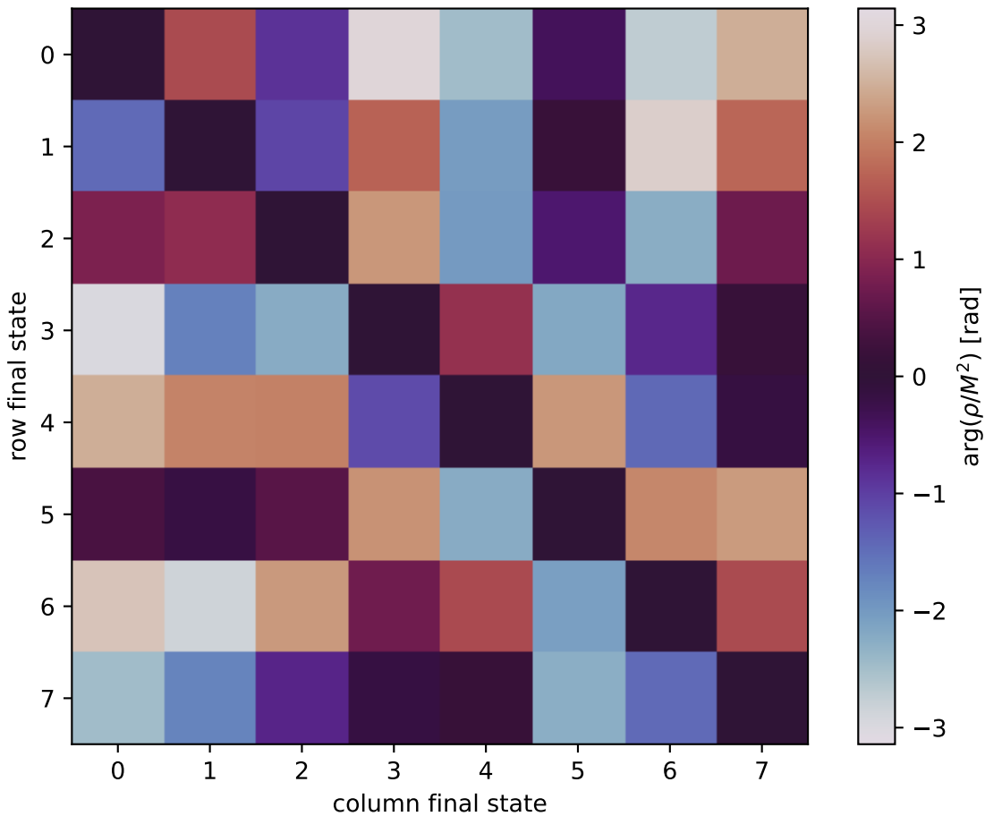
\arg(\rho/M^2) at unpolarized, Q^2=4.5 , t=-1
