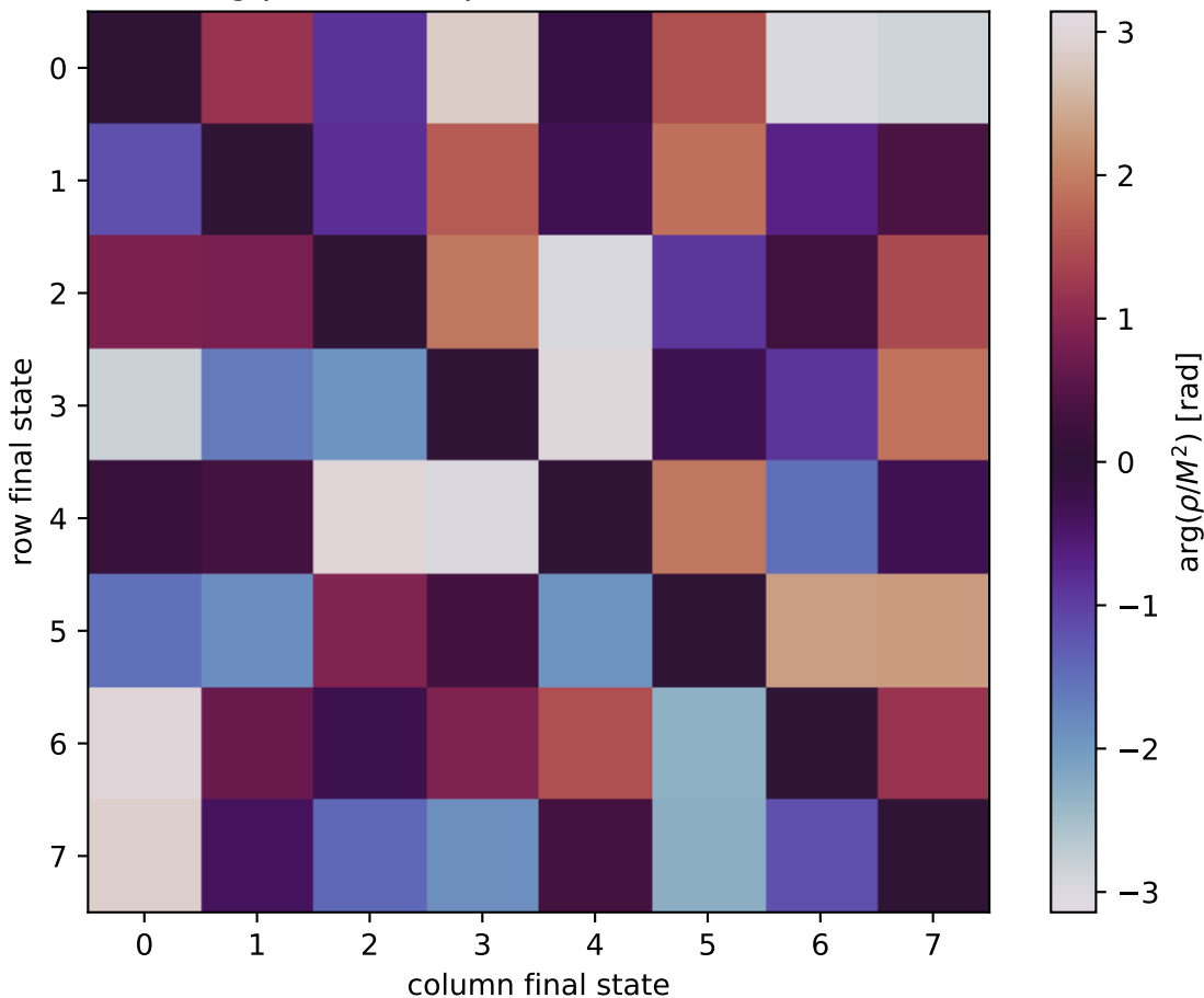
\arg(\rho/M^2) at unpolarized, Q^2=5 , t=-0.6
