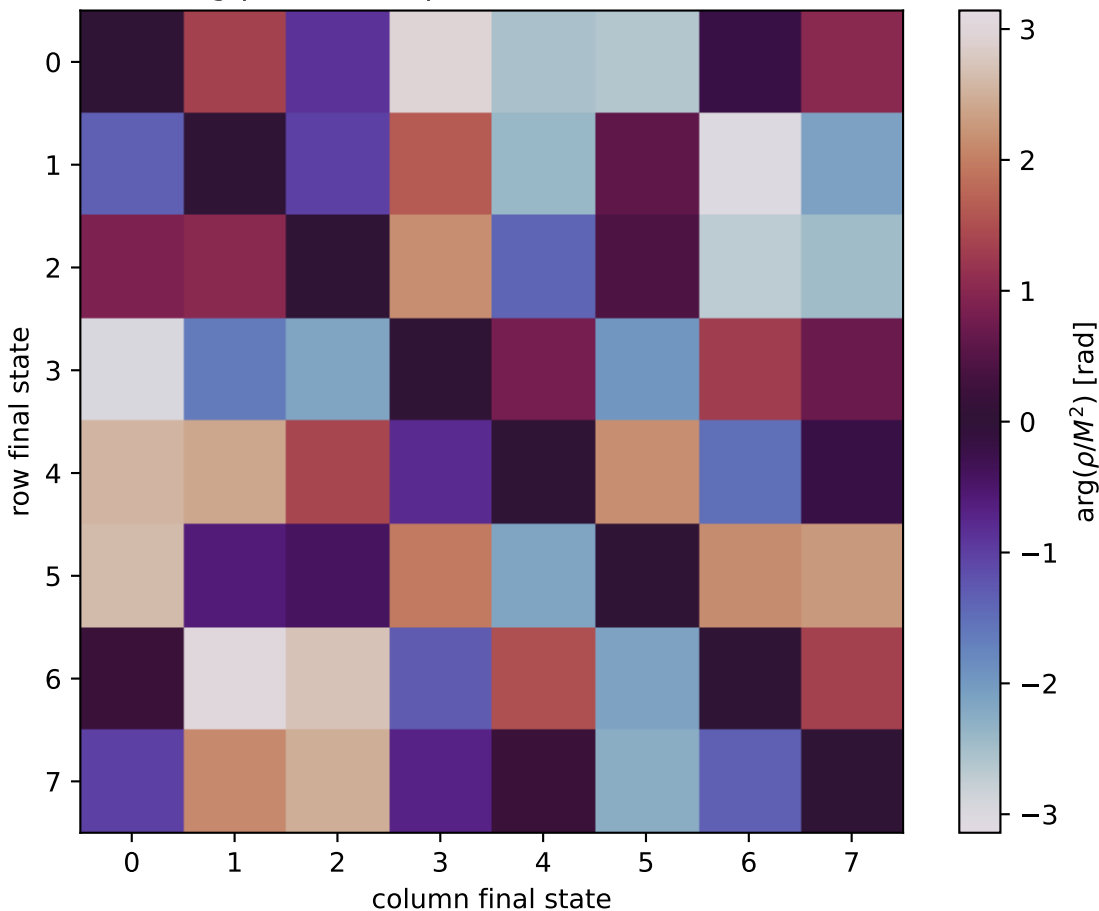
\arg(\rho/M^2) at unpolarized, Q^2=5 , t=-0.8
