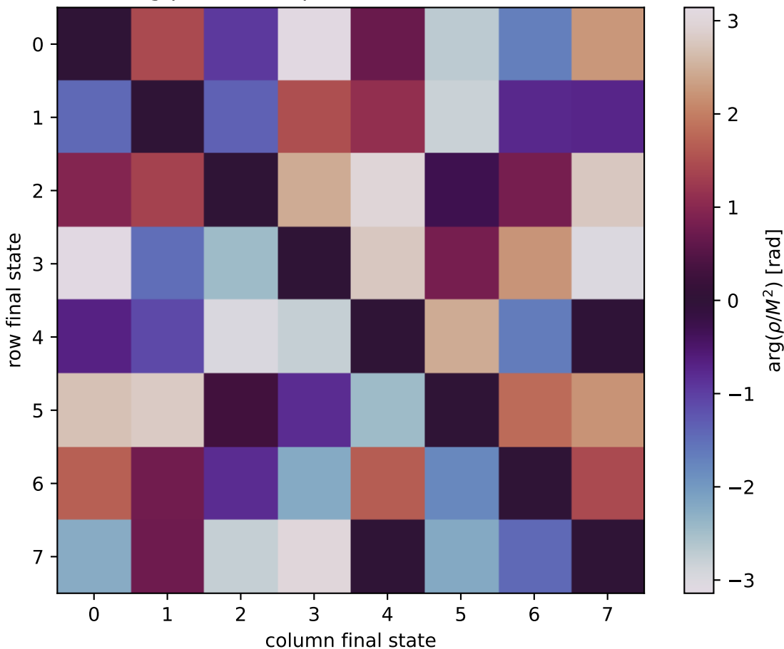
\arg(\rho/M^2) at unpolarized, Q2=5.5, t=-1
