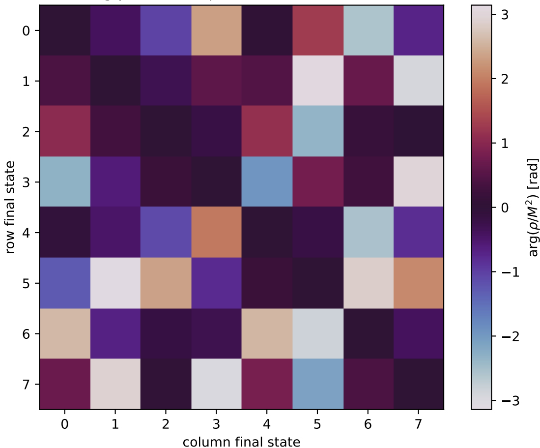
\arg(\rho/M^2) at unpolarized, Q2=6, t=-0.2
