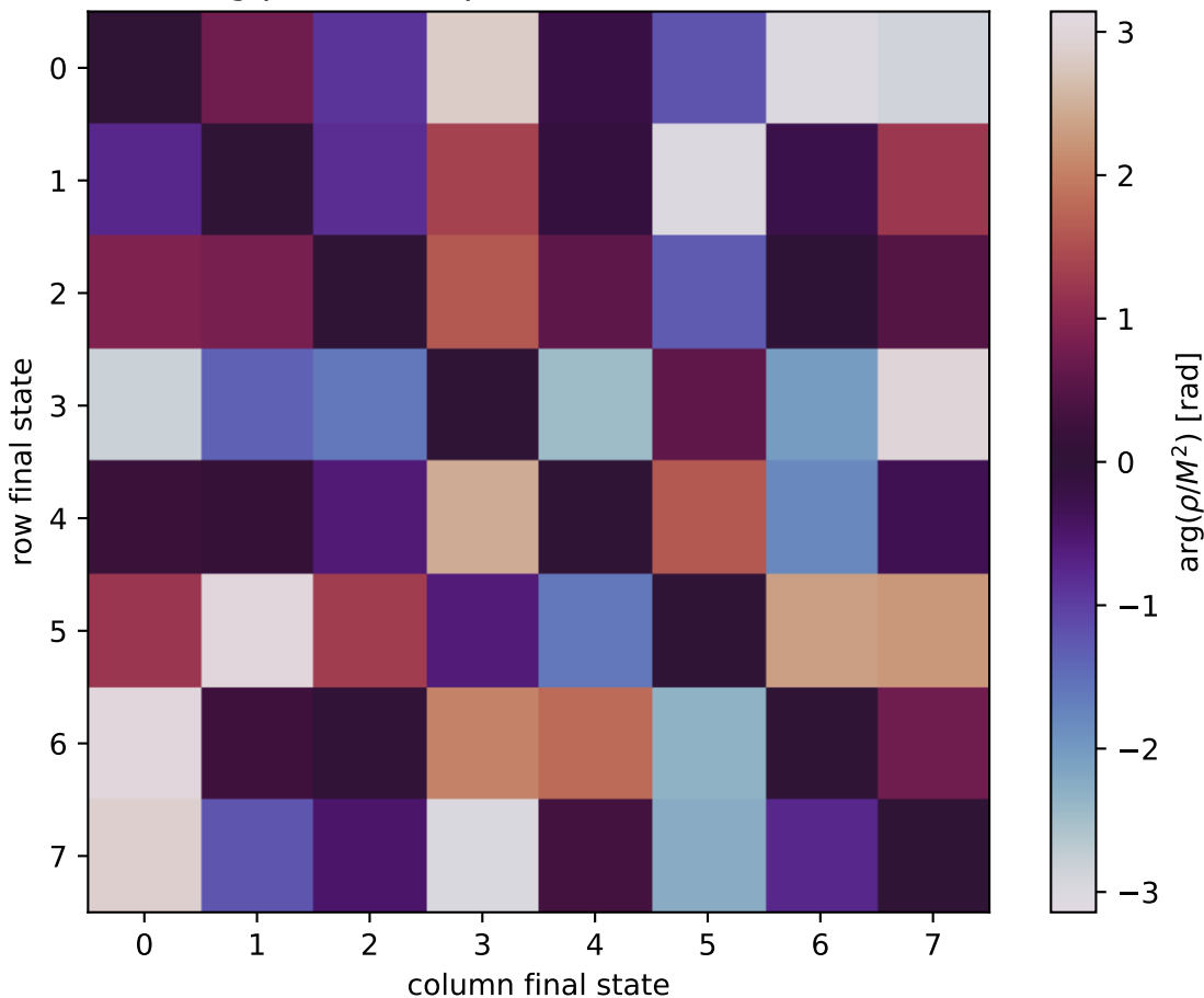
\arg(\rho/M^2) at unpolarized, Q2=6, t=-0.4
