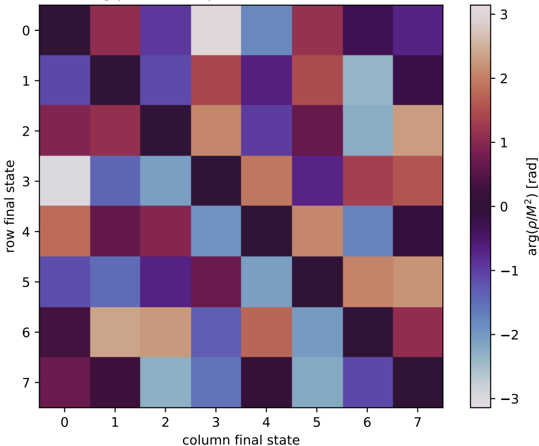
\arg(\rho/M^2) at unpolarized, Q^2=6 , t=-0.6
