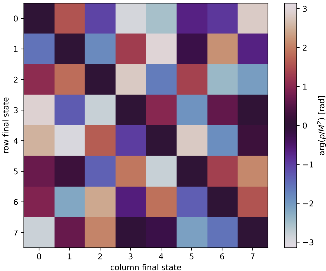
\arg(\rho/M^2) at unpolarized, Q2=6, t=-1.2
