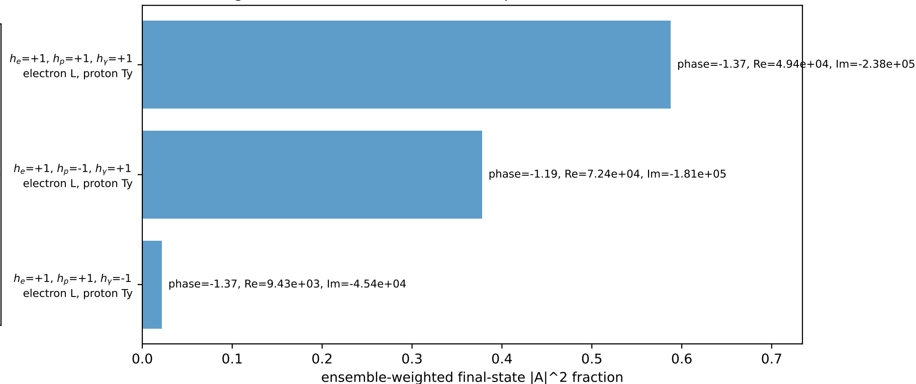
Leading initial-ensemble/final-state components (N=3, retained=98.6%)
