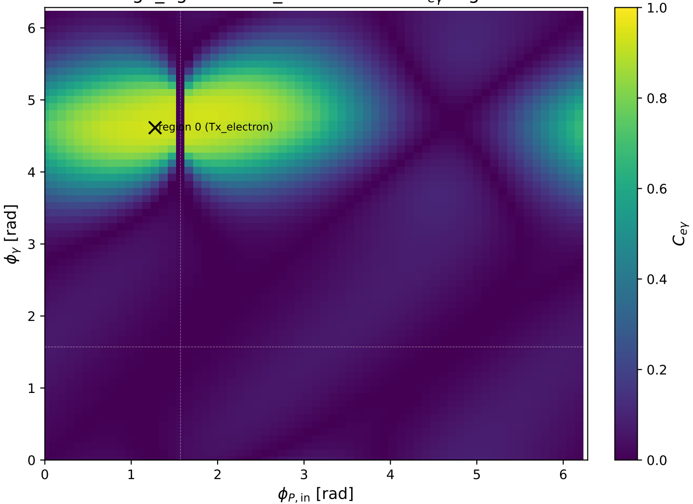
high_Egamma Tx_electron: max C_{e\gamma} regions
