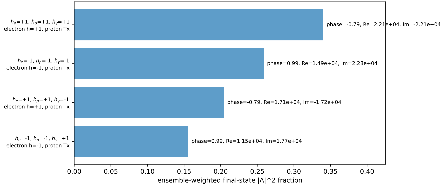
Leading initial-ensemble/final-state components (N=4, retained=95.9%)
