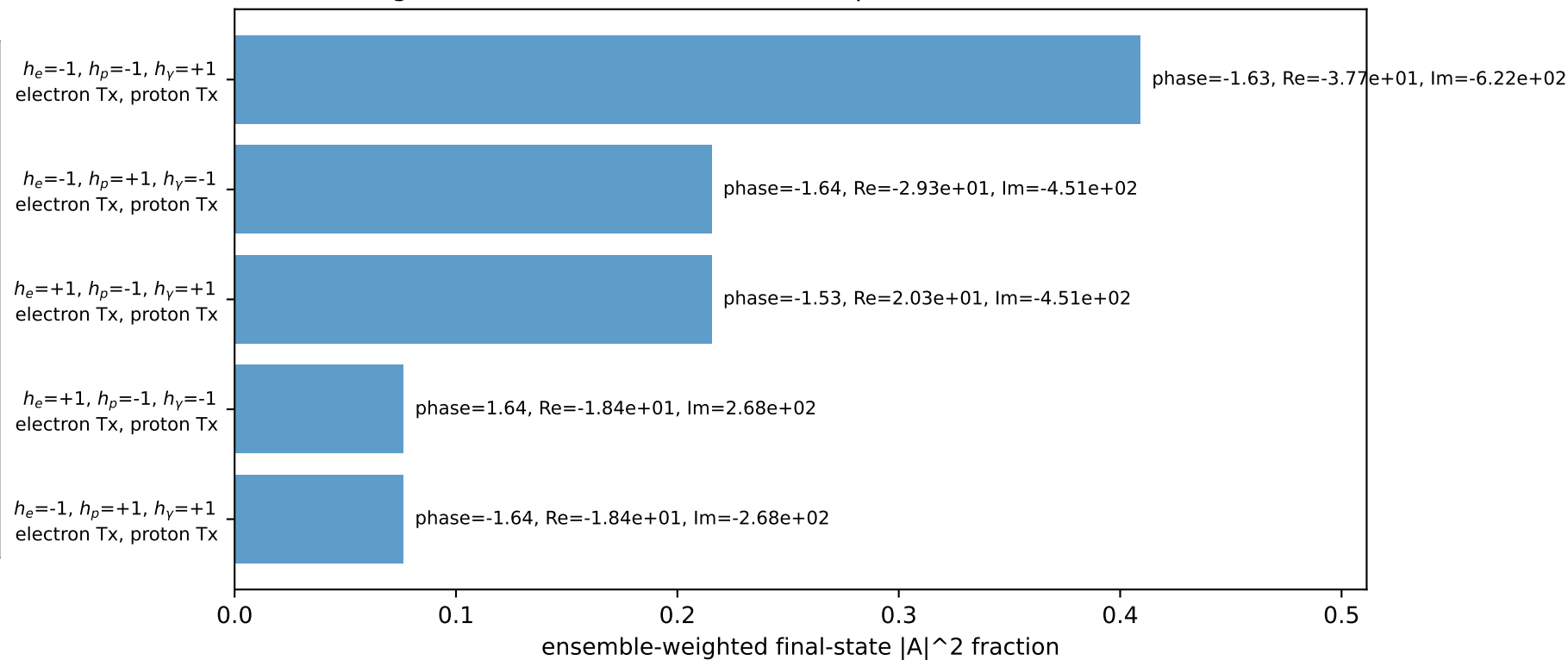
Leading initial-ensemble/final-state components (N=5, retained=99.2%)
