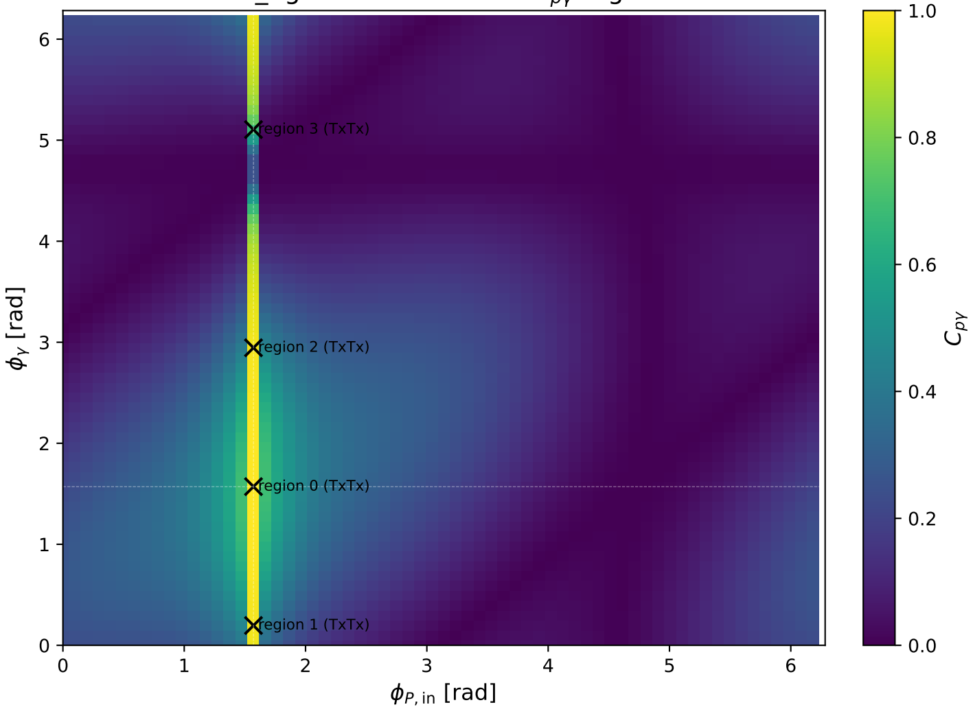
low_Egamma TxTx: max C_{py} regions
