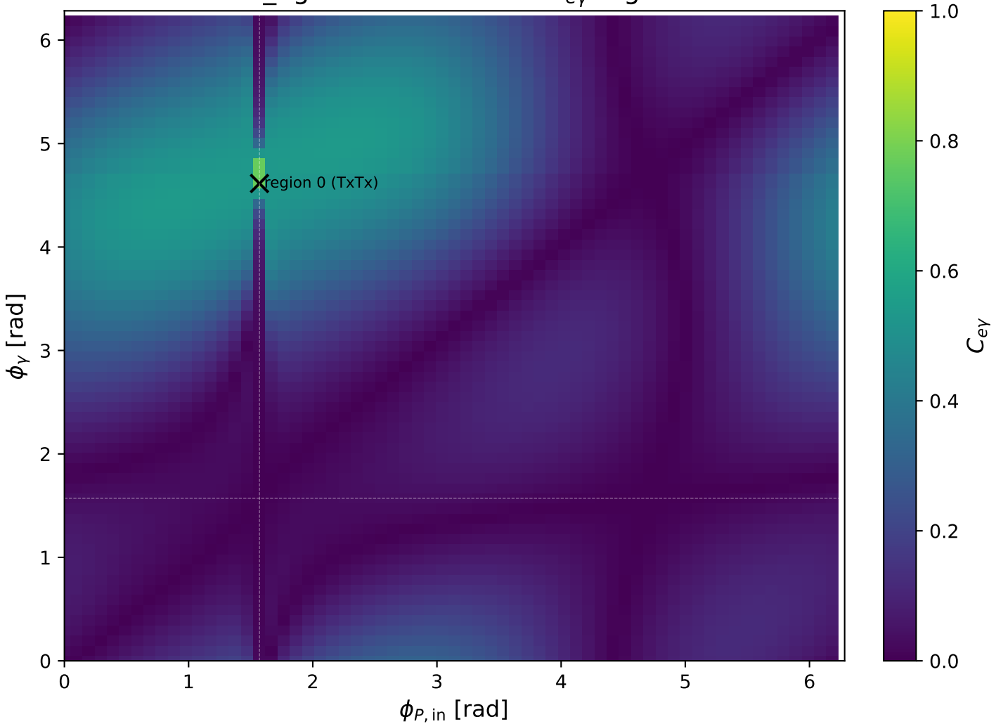
mid_Egamma TxTx: max C_{ey} regions
