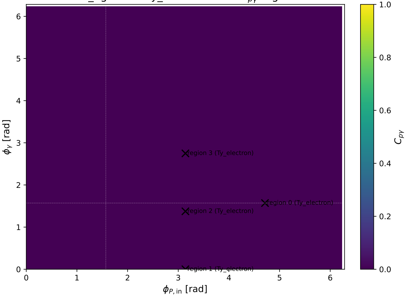
low_Egamma Ty_electron: max C_{p\gamma} regions
