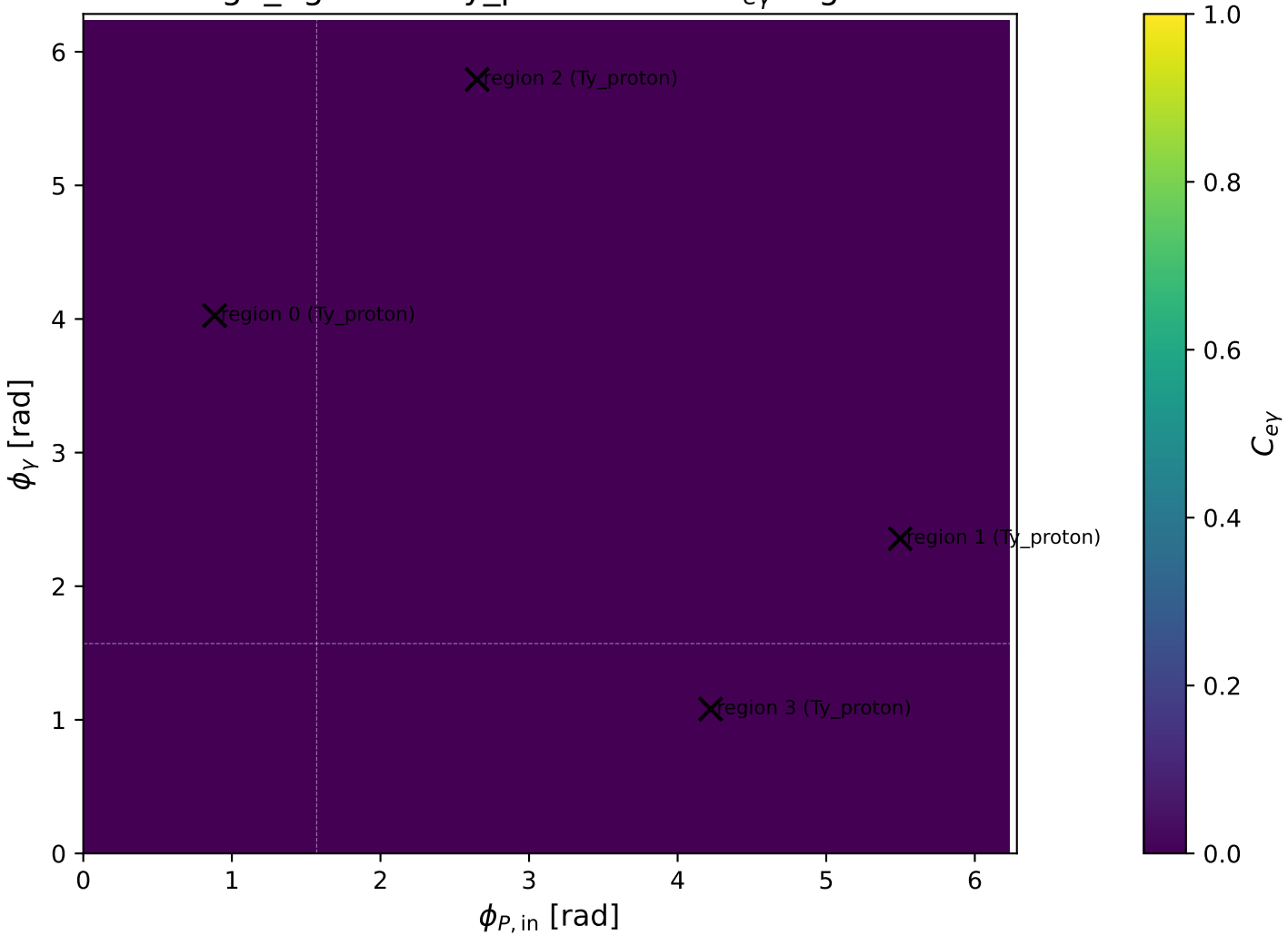
high_Egamma Ty_proton: max C_{ey} regions
