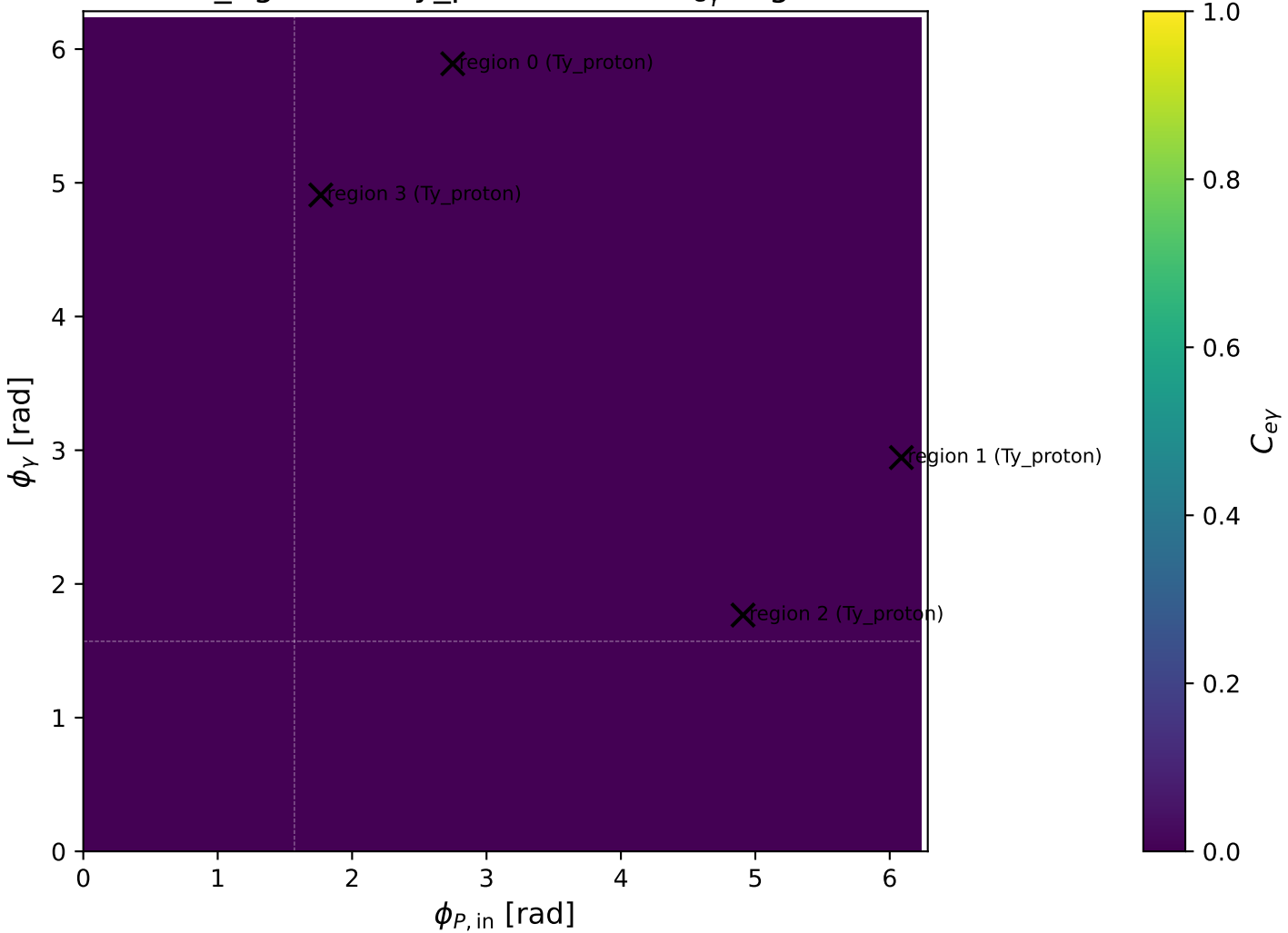
mid_Egamma Ty_proton: max C_{e\gamma} regions
