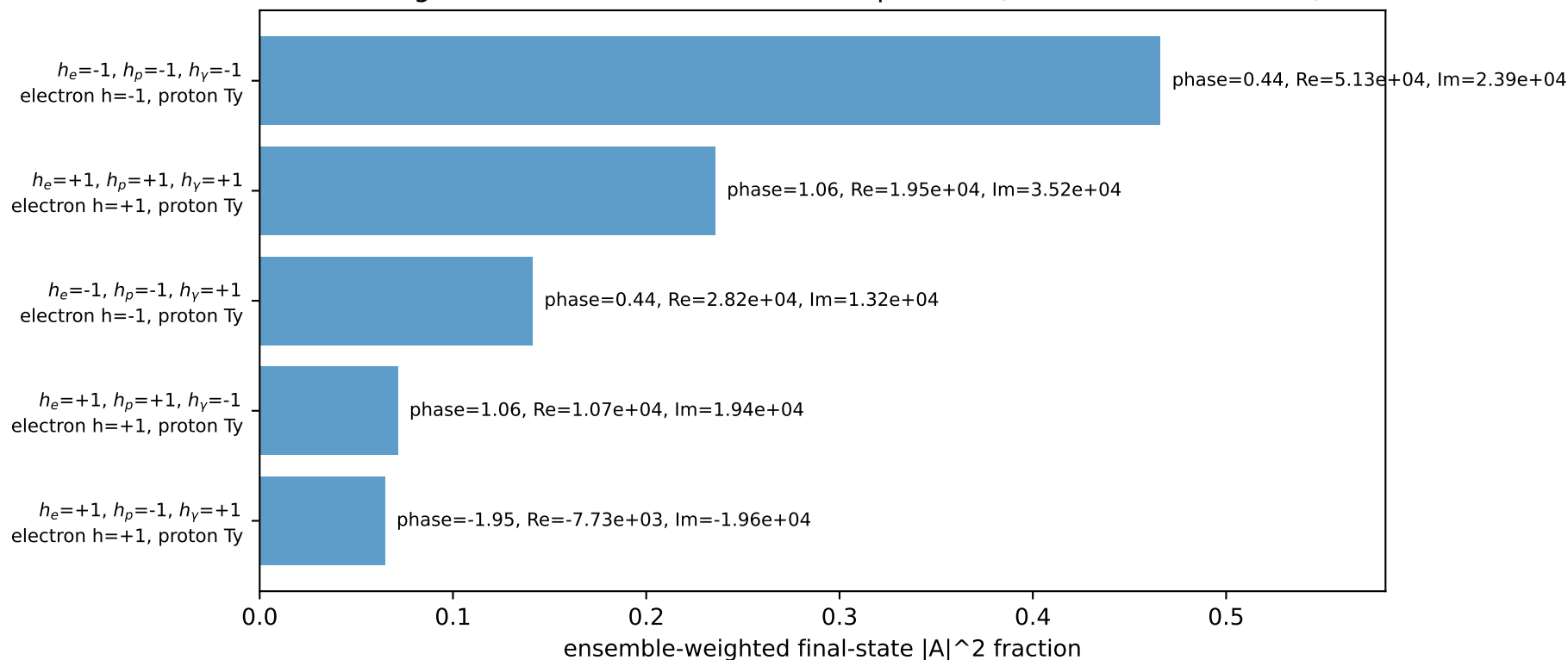
Leading initial-ensemble/final-state components (N=5, retained=97.9%)
