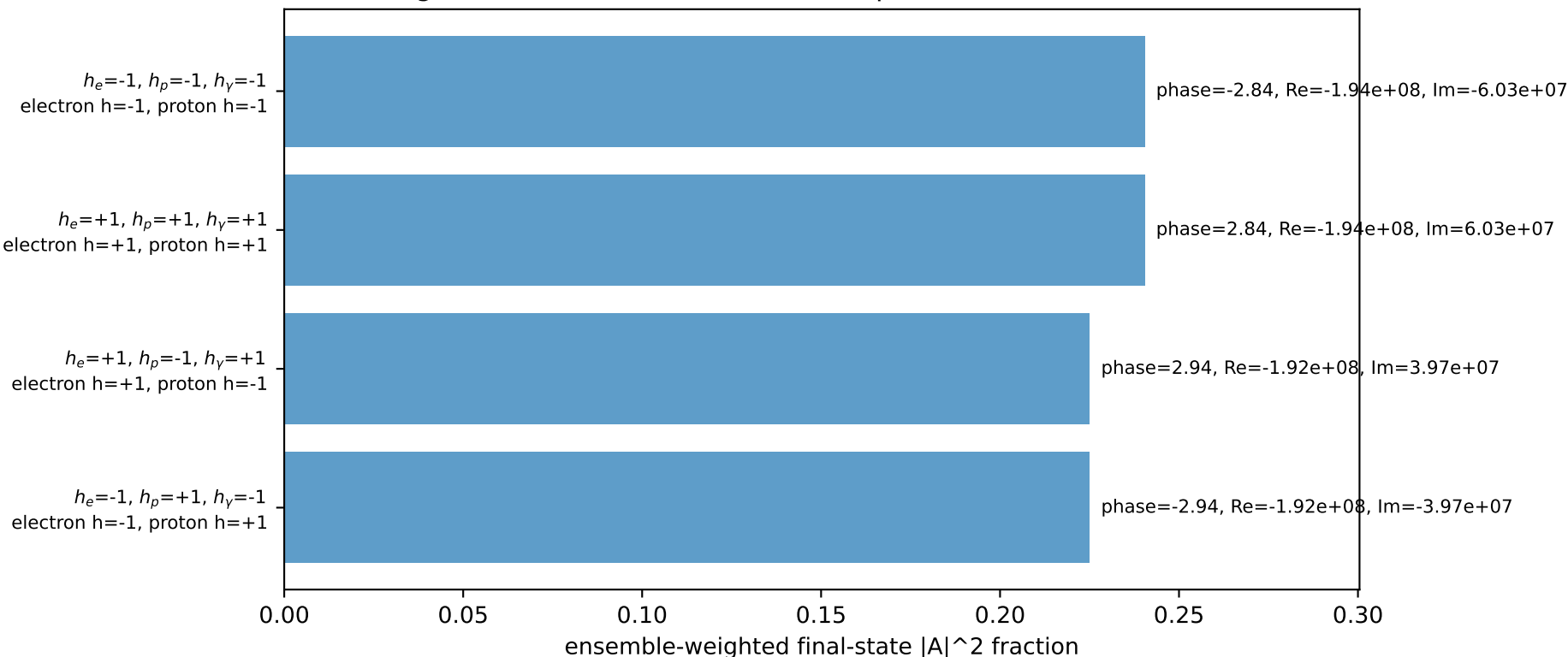
Leading initial-ensemble/final-state components (N=4, retained=93.1%)
