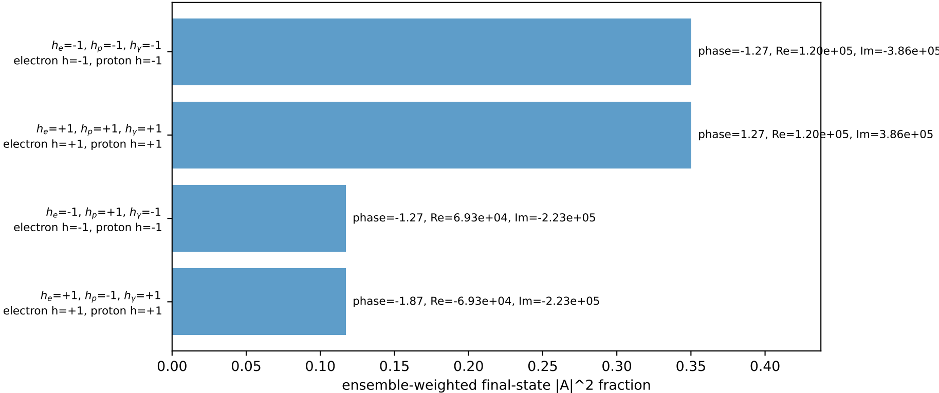
Leading initial-ensemble/final-state components (N=4, retained=93.4%)
