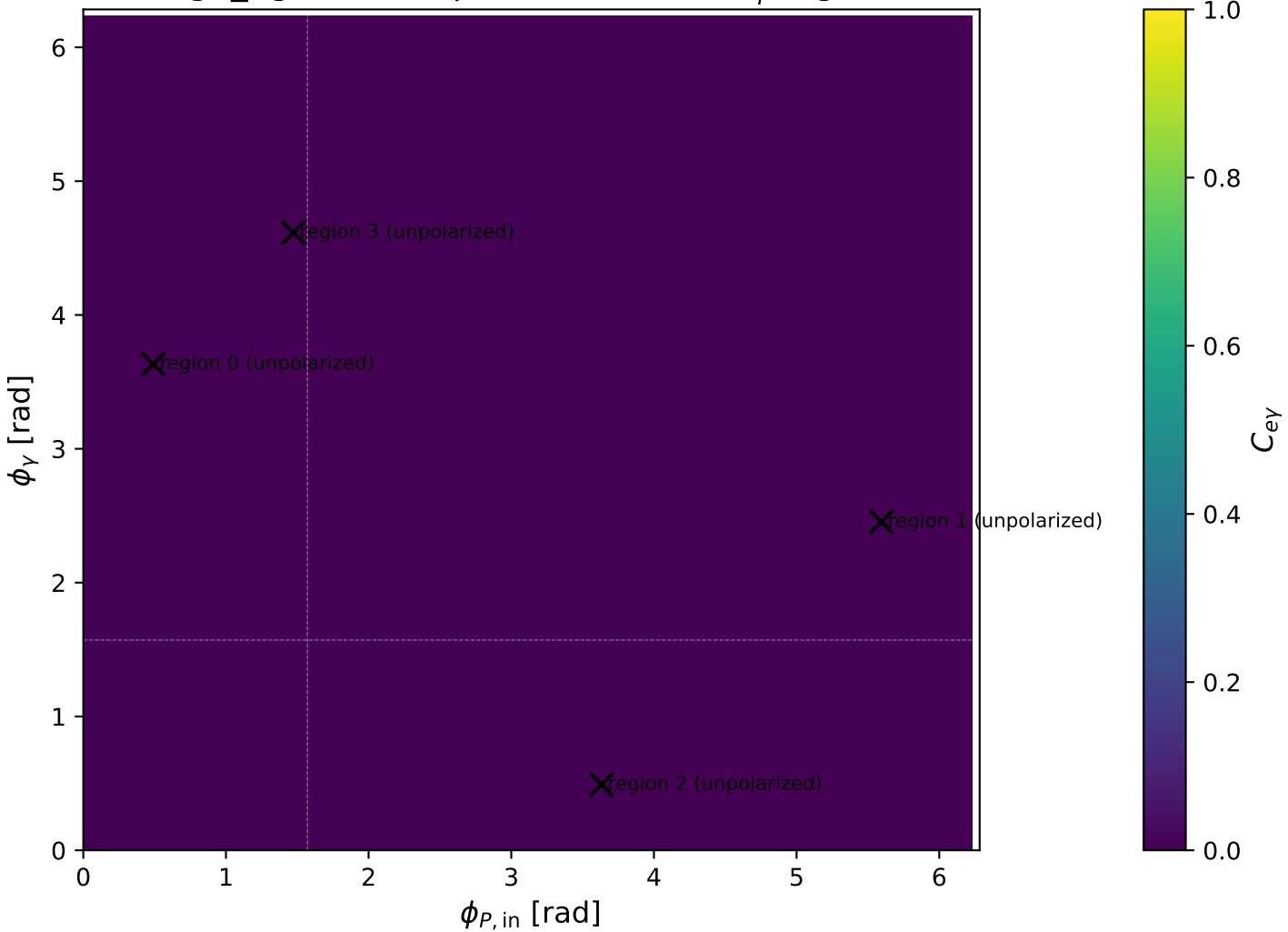
high_Egamma unpolarized: max C_{ey} regions
