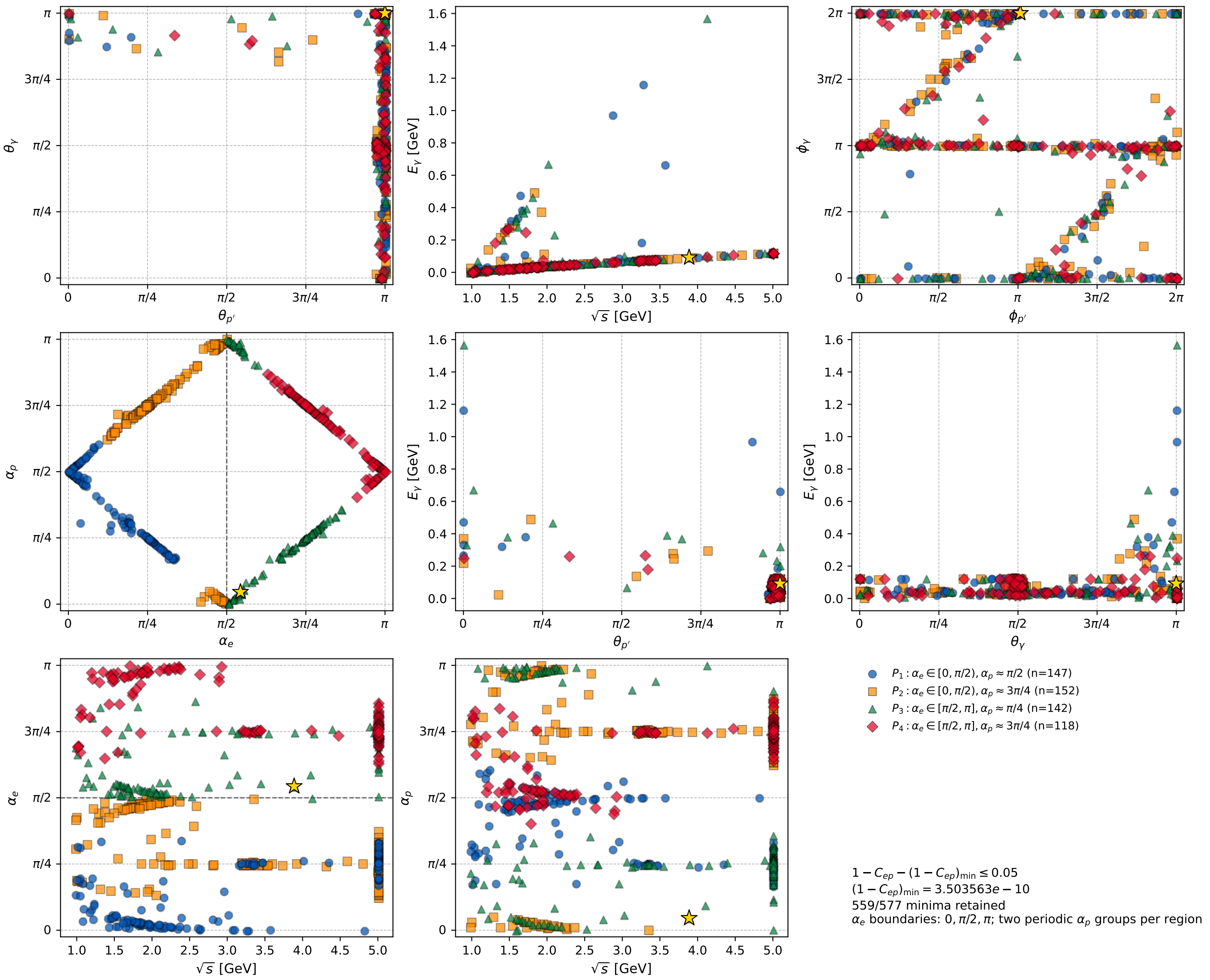
electron: low-1 – C_{ep} phase space colored by 4 major polarization configurations
