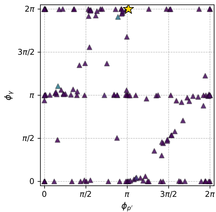
electron: polarization cluster P3; all member minima in phase space
