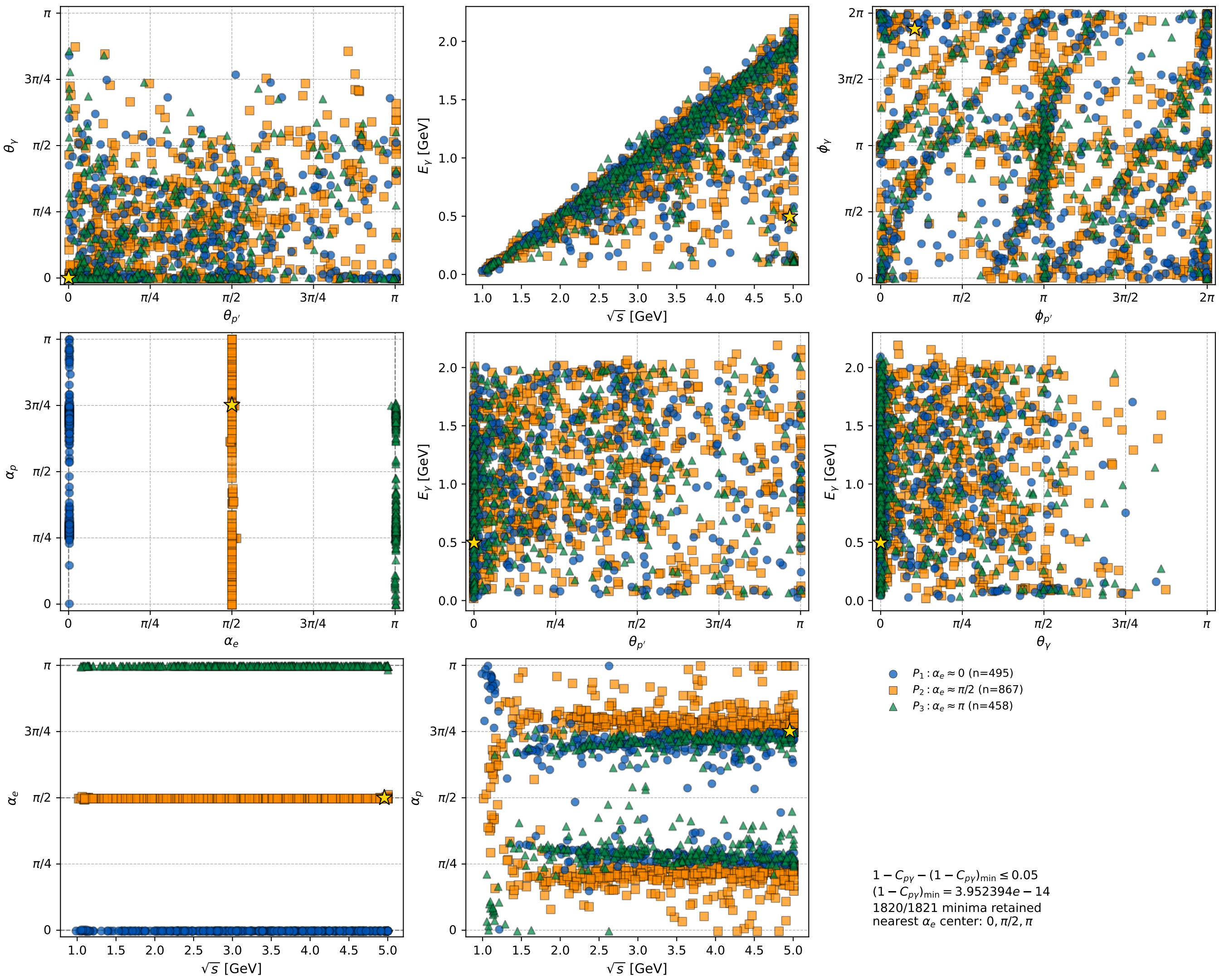
electron: low-1 - C_{p\gamma} phase space colored by 3 major polarization configurations
