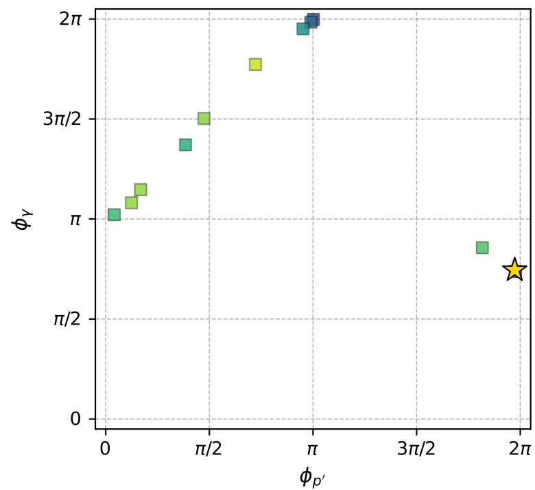
muon: polarization cluster P2; all member minima in phase space
