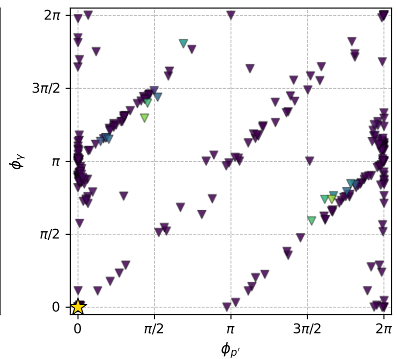
muon: polarization cluster P5; all member minima in phase space
