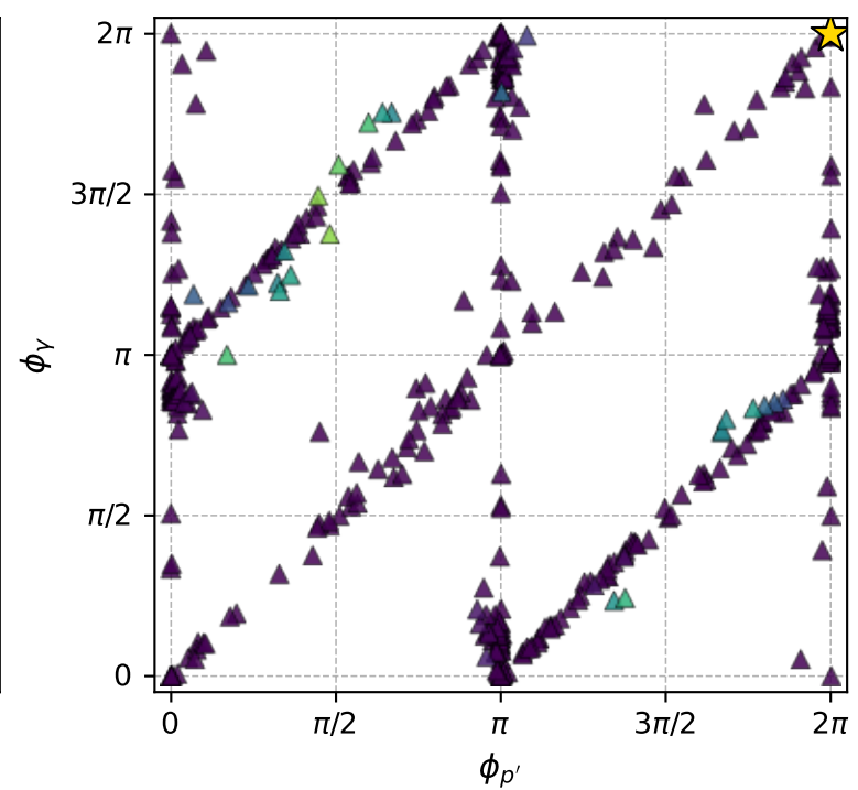
muon: polarization cluster P3; all member minima in phase space
