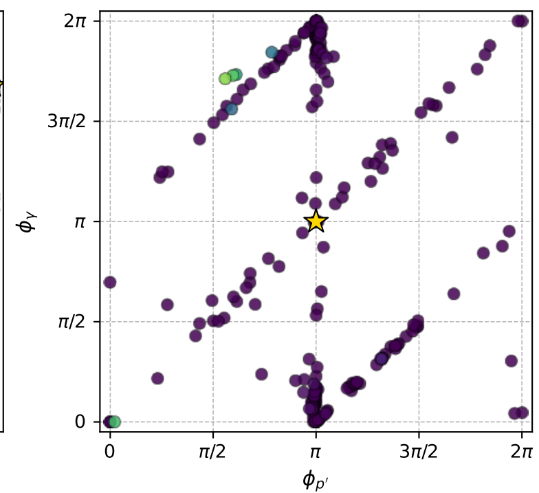
muon: polarization cluster P1; all member minima in phase space
