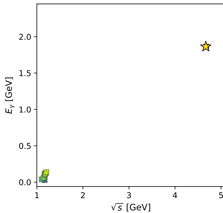
muon: polarization cluster P2; all member minima in phase space
