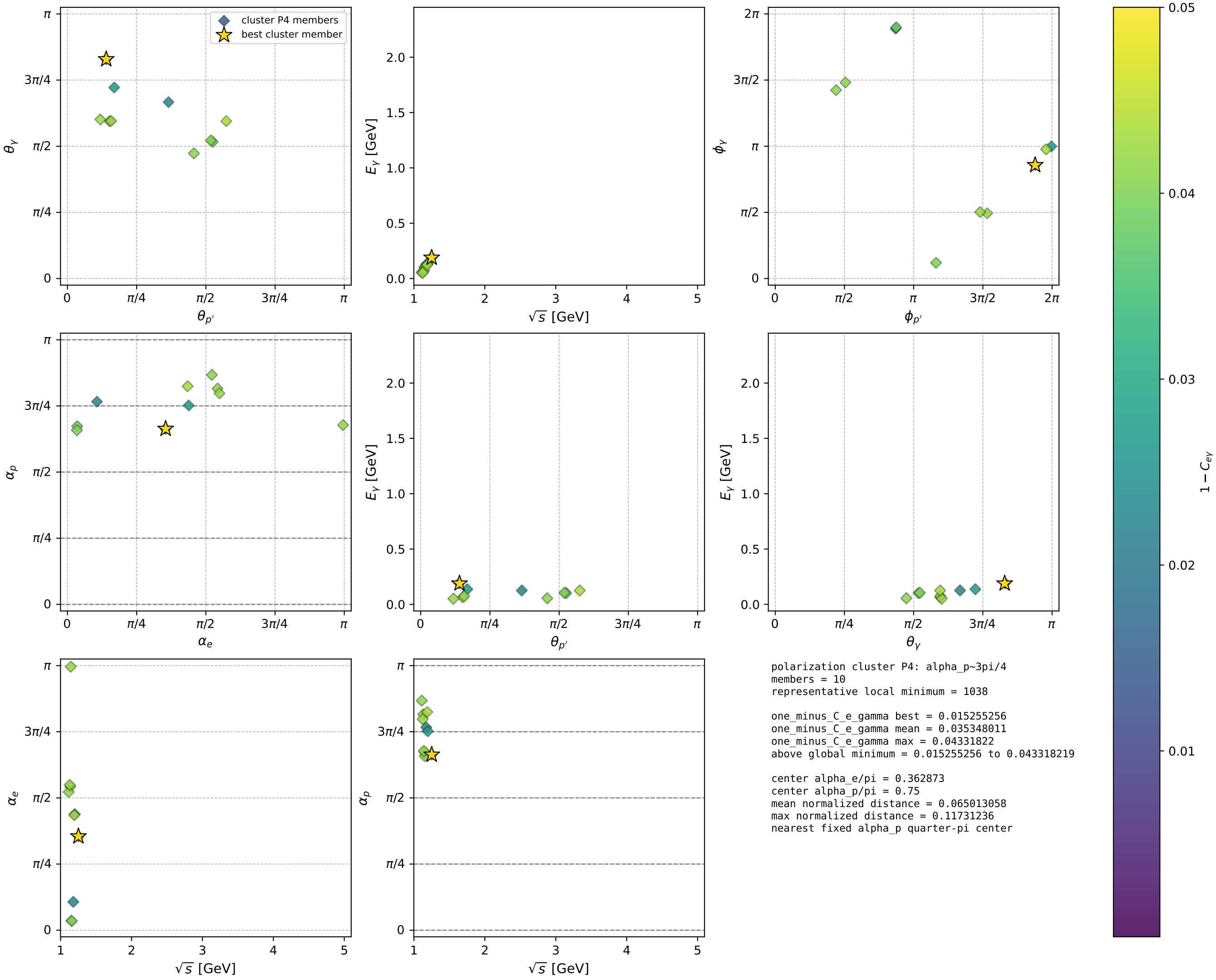
muon: polarization cluster P4; all member minima in phase space
