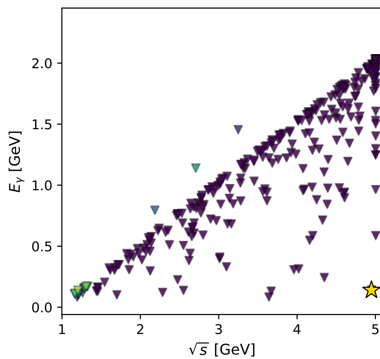
muon: polarization cluster P5; all member minima in phase space
