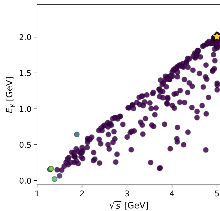
muon: polarization cluster P1; all member minima in phase space
