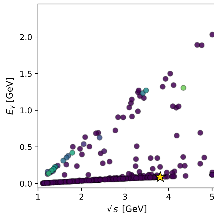
muon: polarization cluster P1; all member minima in phase space
