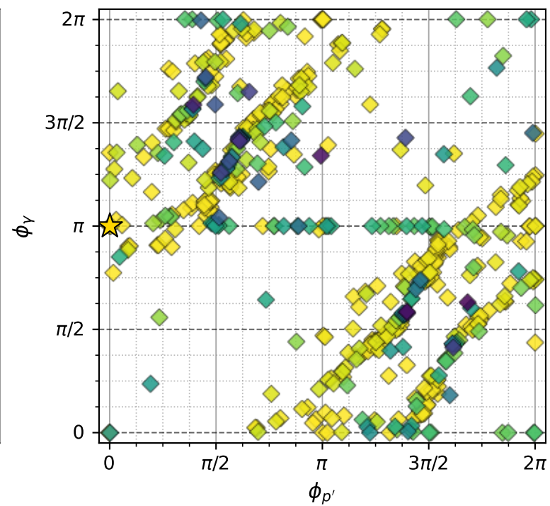
muon: polarization cluster P4; all member minima in phase space
