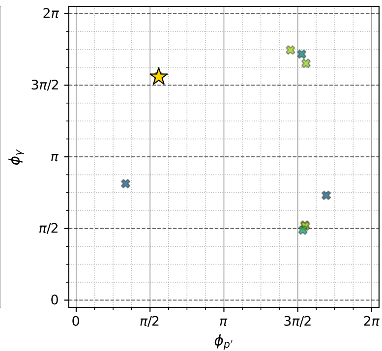
muon: polarization cluster P6; all member minima in phase space
