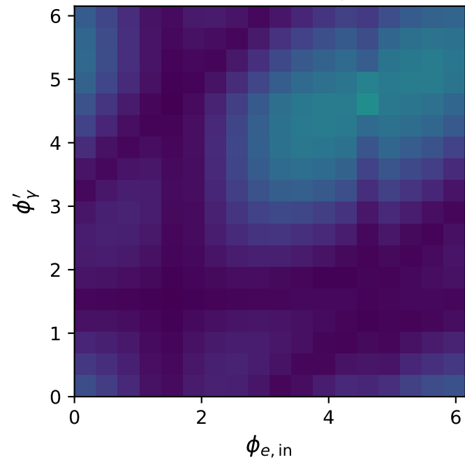
high_s, high_theta_in low_Egamma, max C_{e\gamma} =0.672
