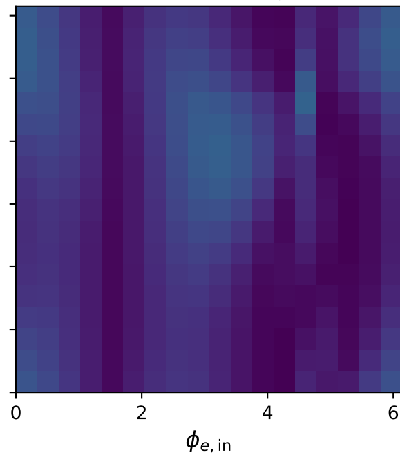
high_s, high_theta_in mid_Egamma, max C_{ep} =0.611
