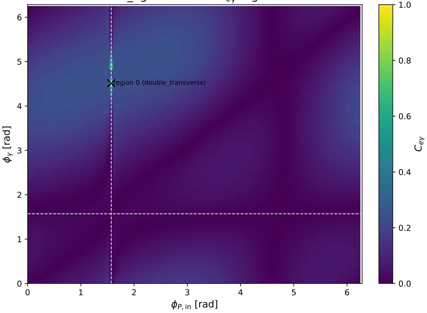
low_Egamma: max C_{e\gamma} regions
