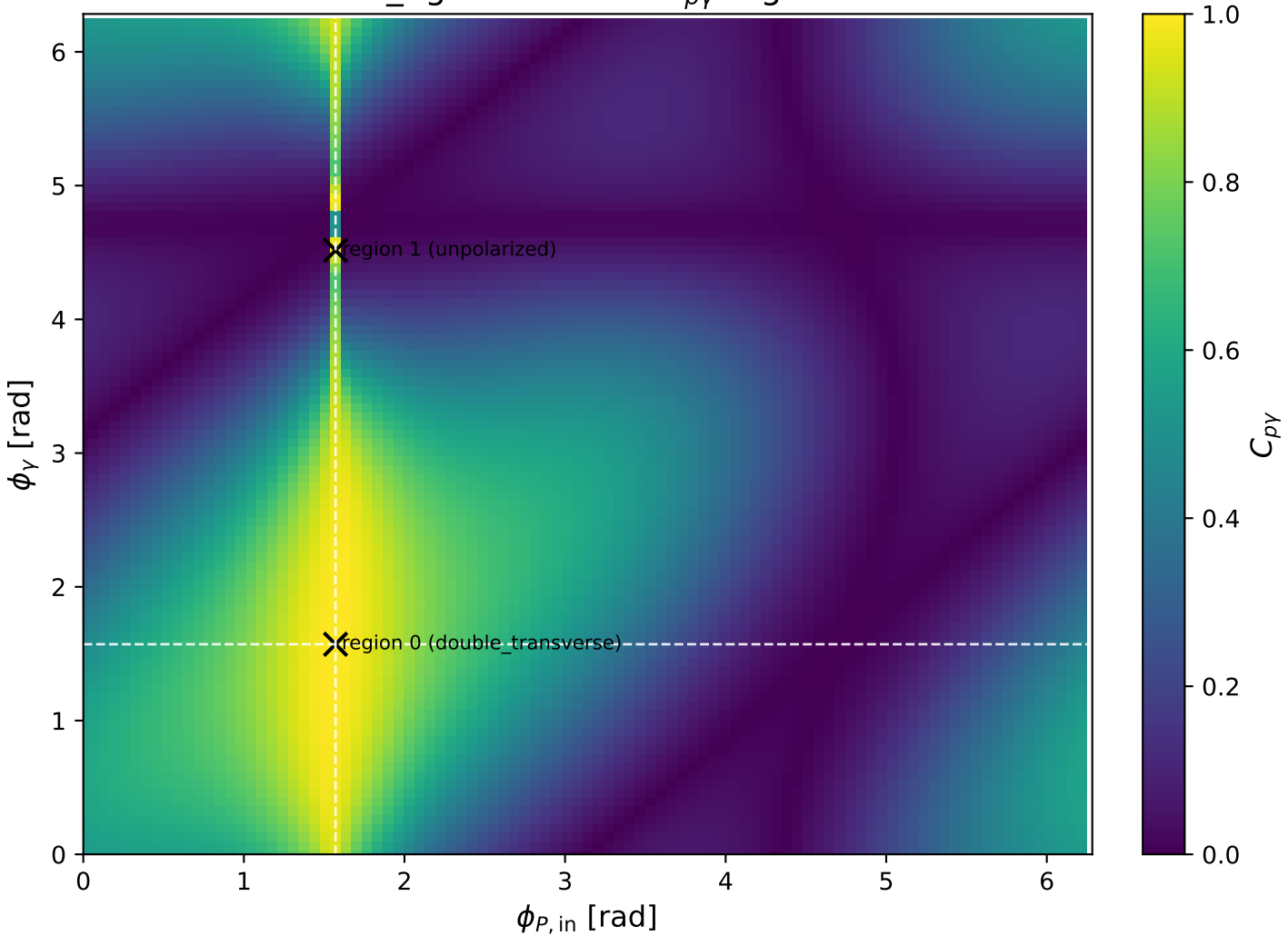
mid_Egamma: max C_{p\gamma} regions
