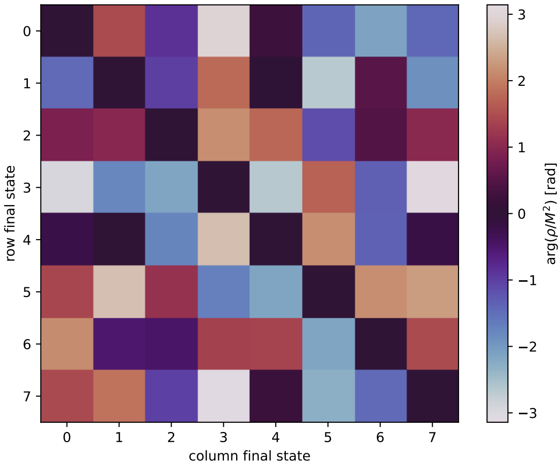
\arg(\rho/M^2) at Q2=4, t=-1
