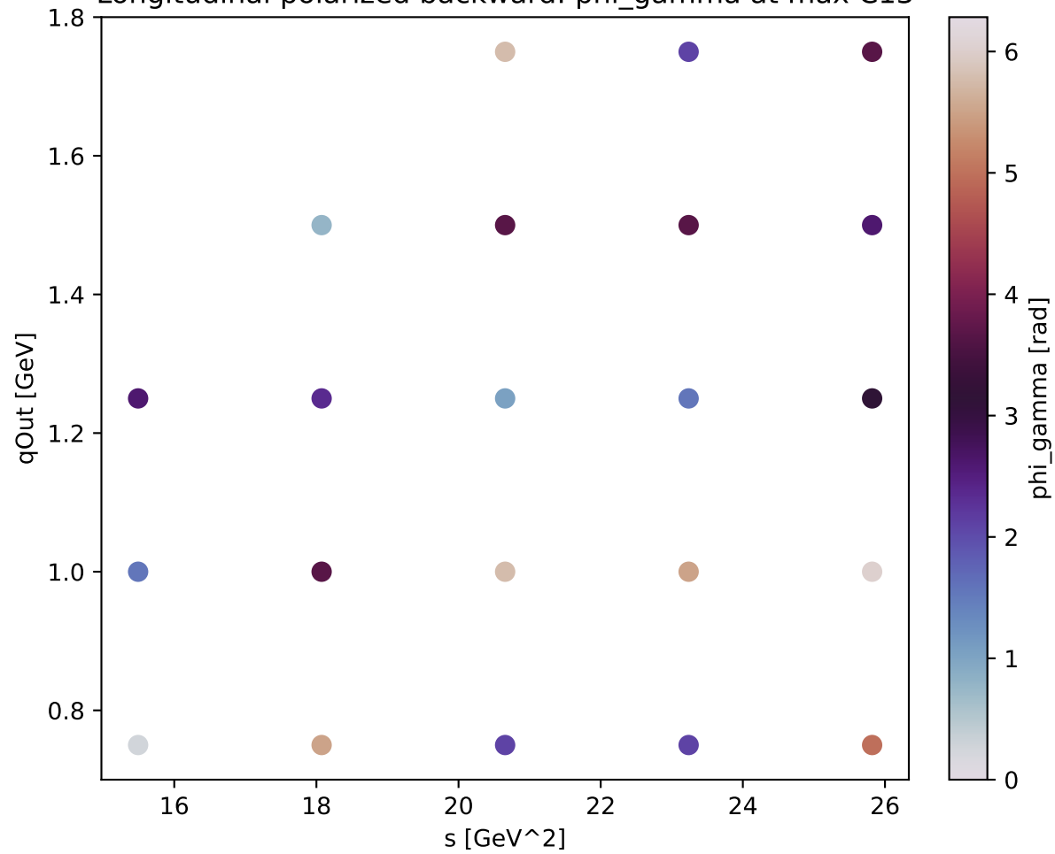
Longitudinal polarized backward: phi_gamma at max C13
