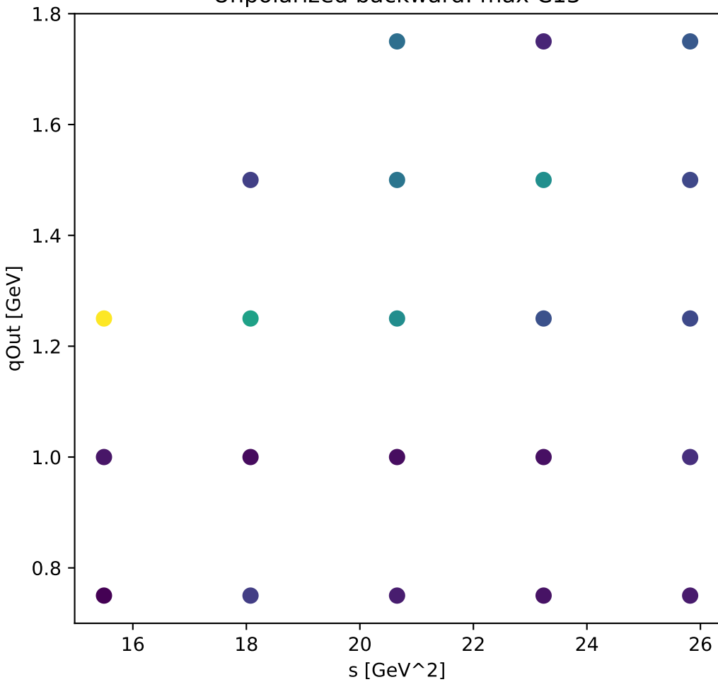
Unpolarized backward: max C13
