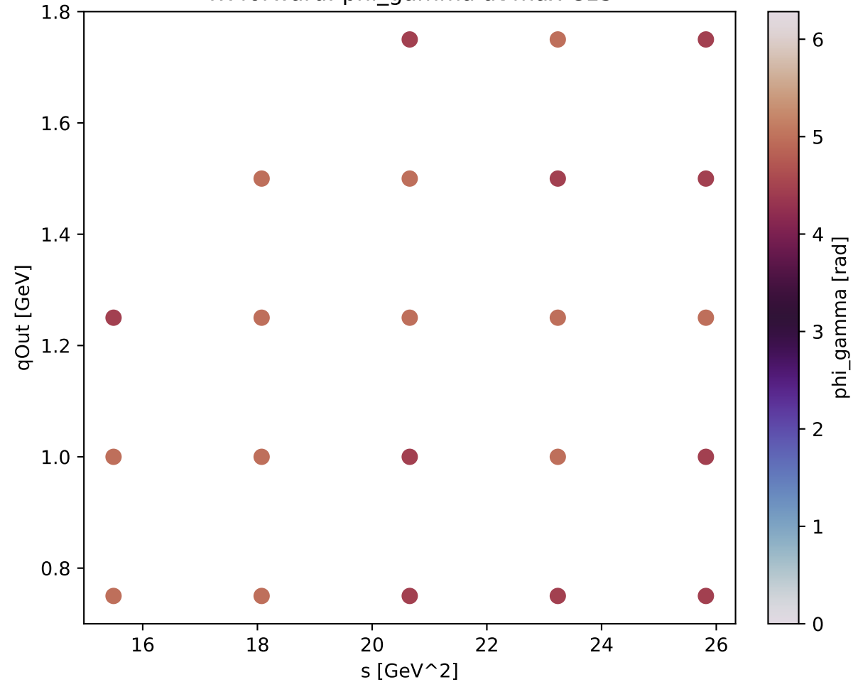
Tx forward: phi_gamma at max C13
