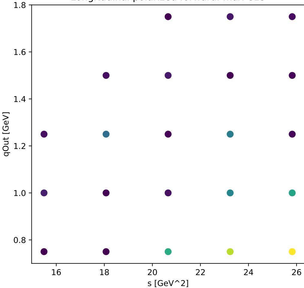
Longitudinal polarized forward: max C13
