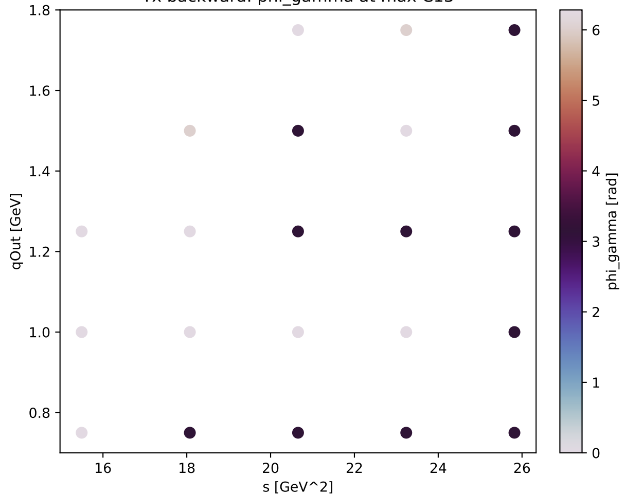
Tx backward: phi_gamma at max C13
