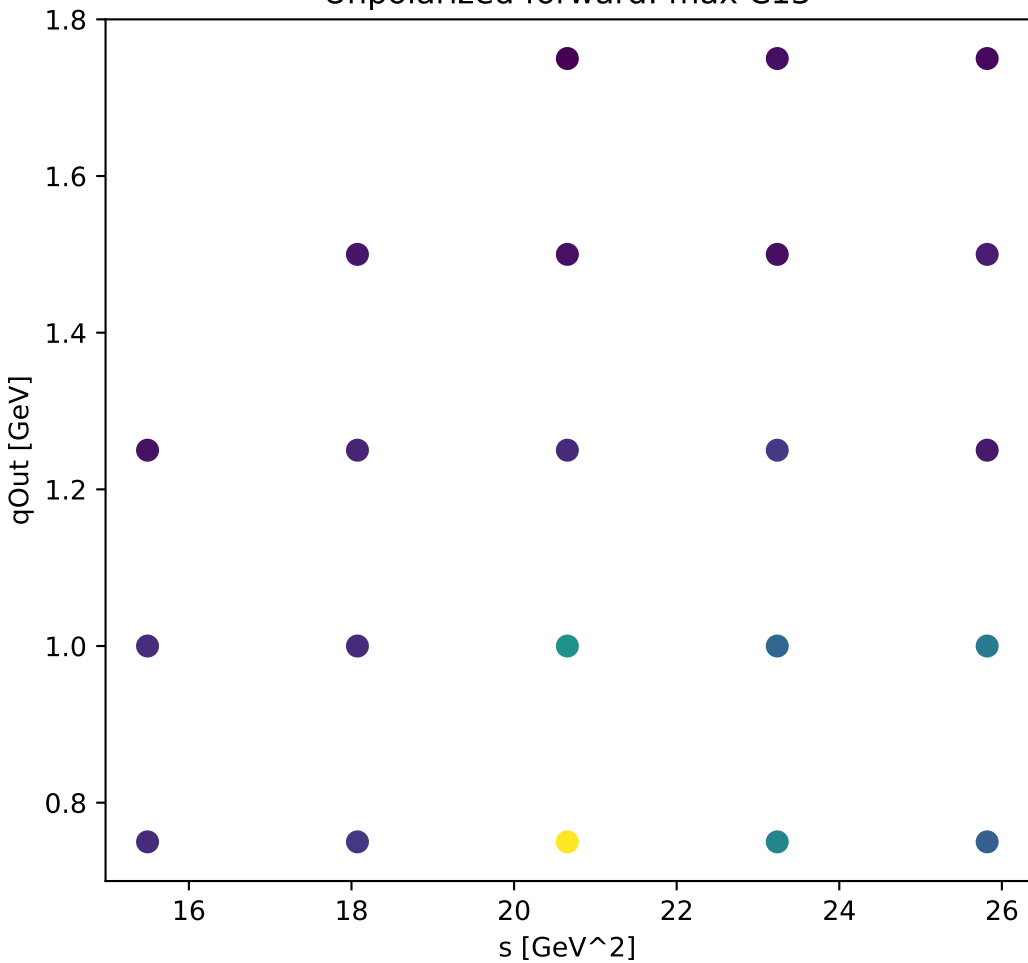
Unpolarized forward: max C13
