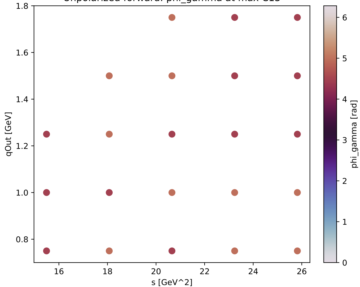
Unpolarized forward: phi_gamma at max C13
