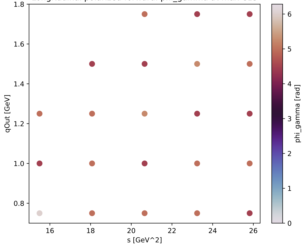
Longitudinal polarized forward: phi_gamma at max C13
