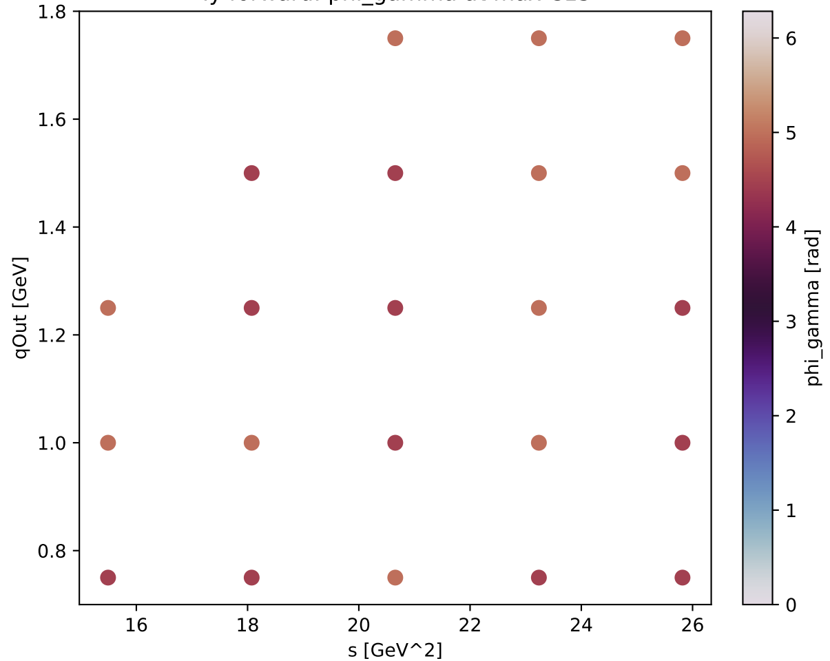
Ty forward: phi_gamma at max C13
