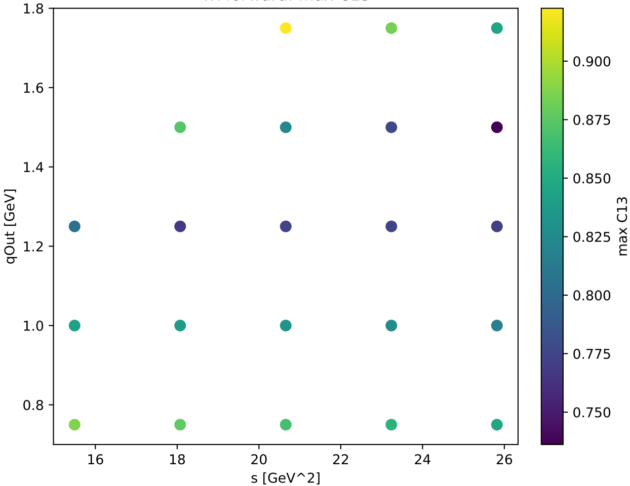
Tx forward: max C13
