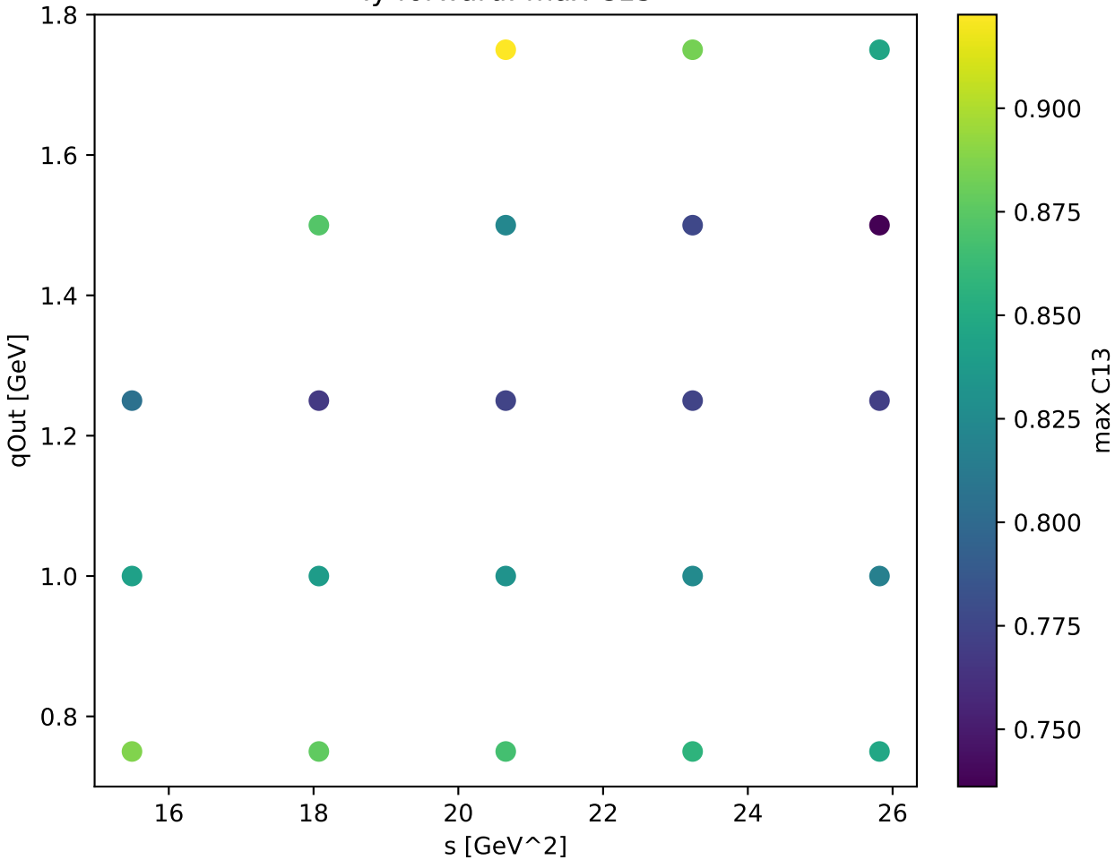
Ty forward: max C13
