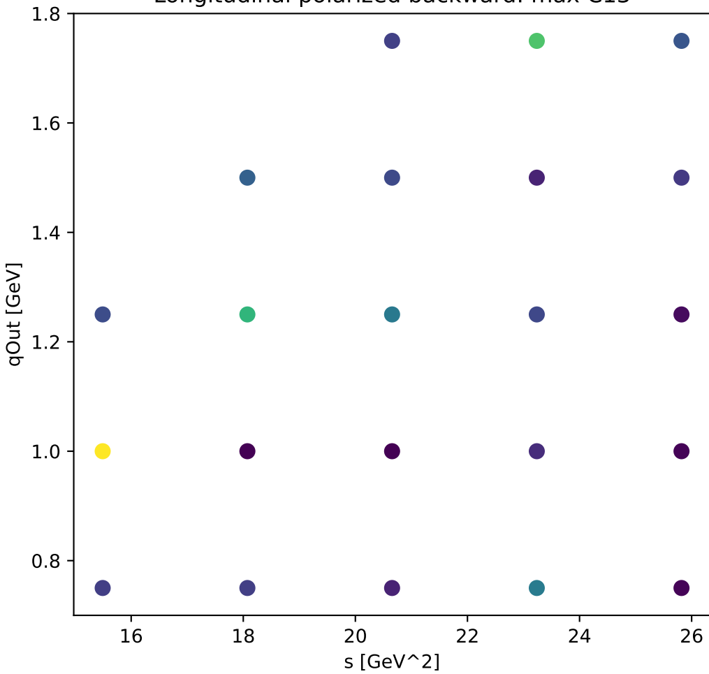
Longitudinal polarized backward: max C13
