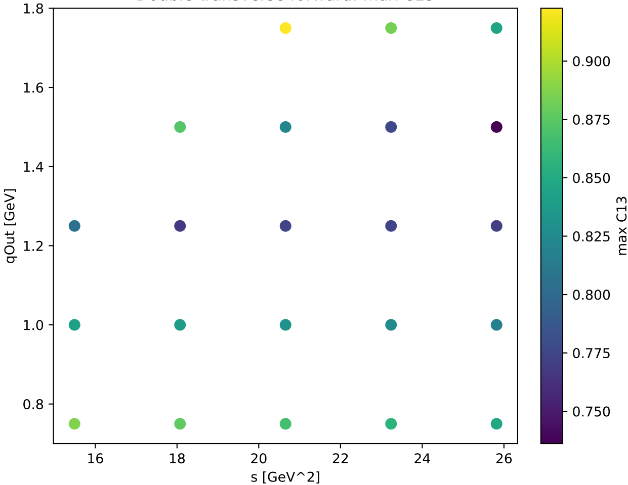
Double transverse forward: max C13
