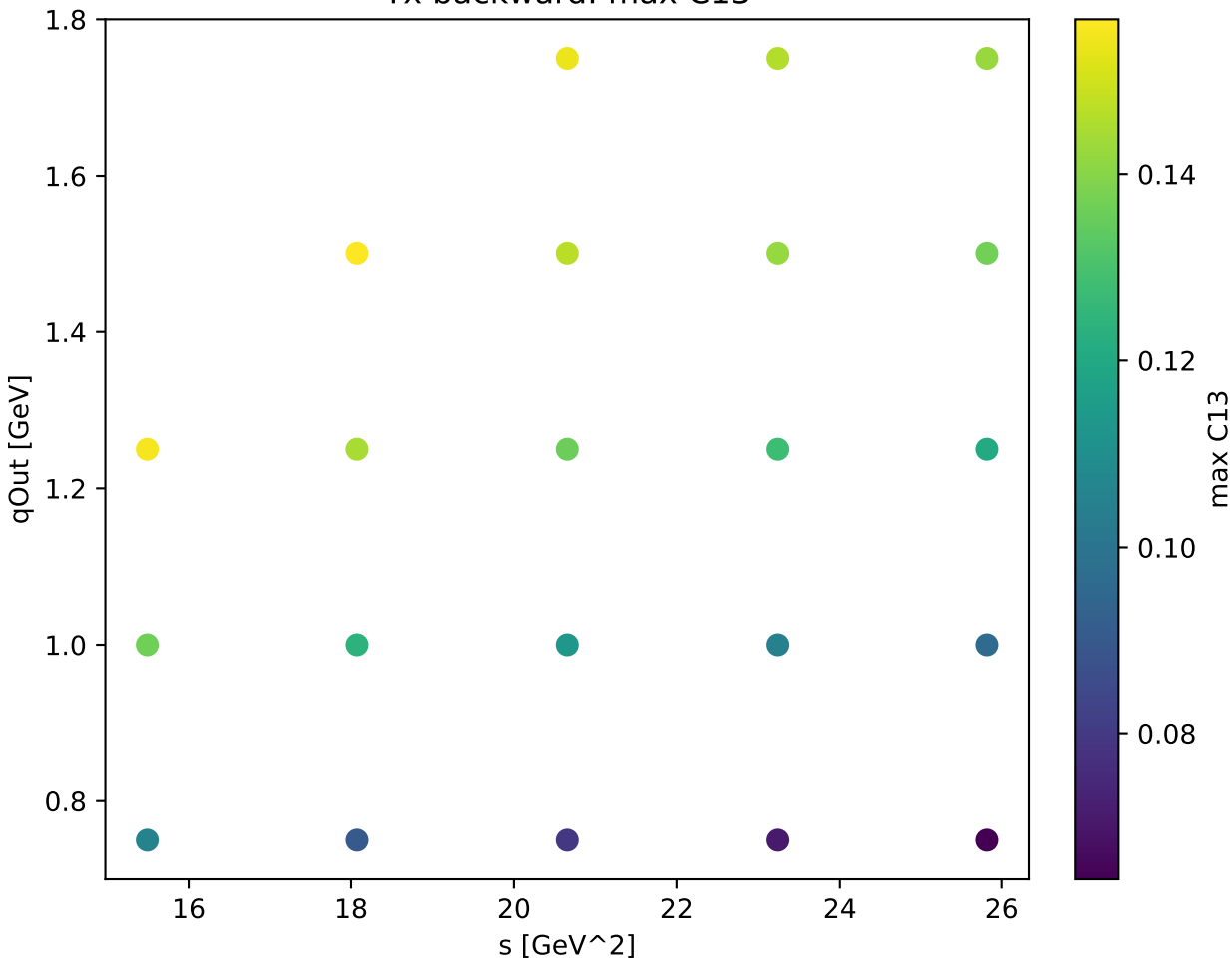
Tx backward: max C13
