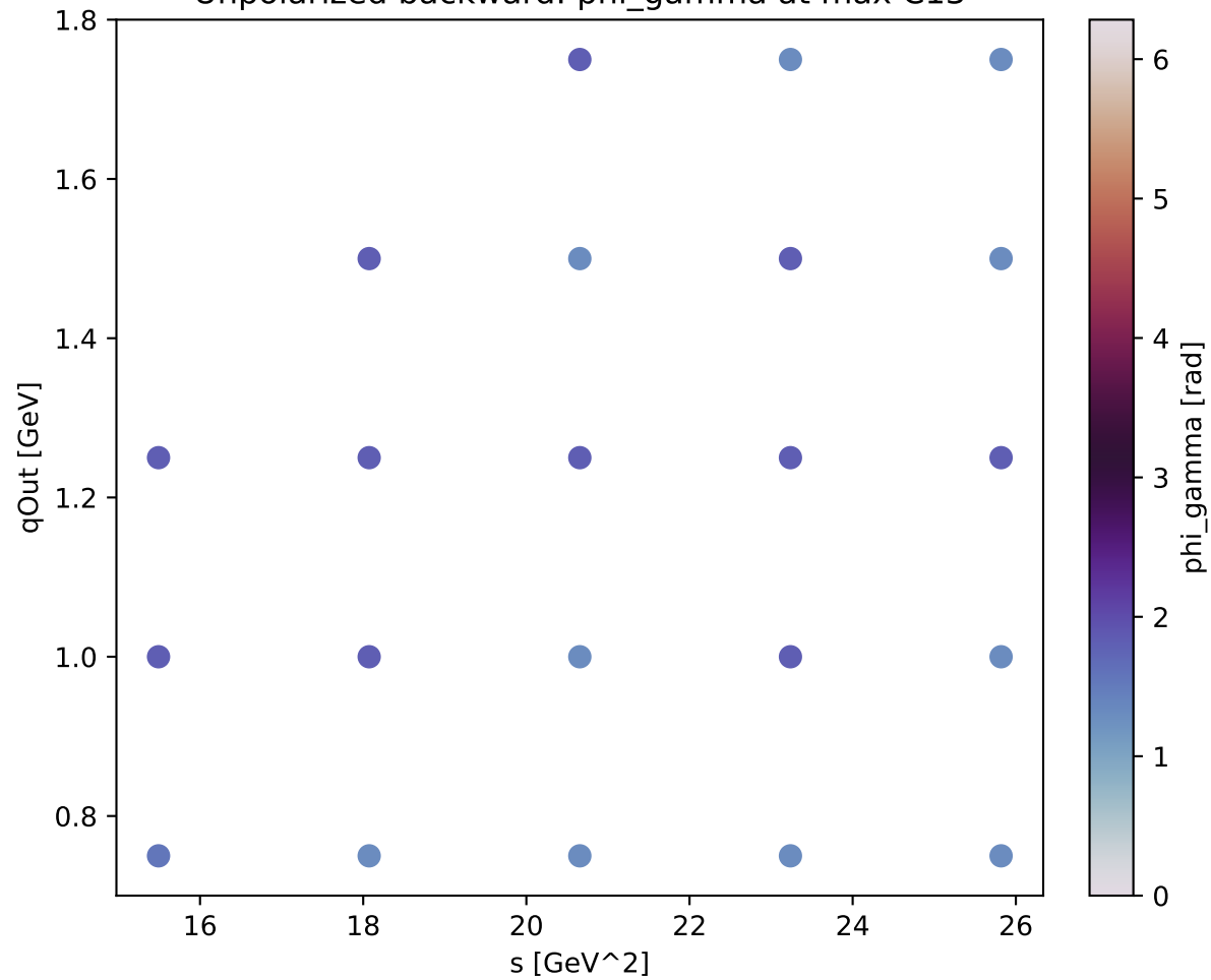
Unpolarized backward: phi_gamma at max C13
