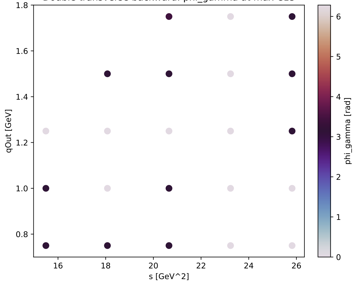
Double transverse backward: phi_gamma at max C13
