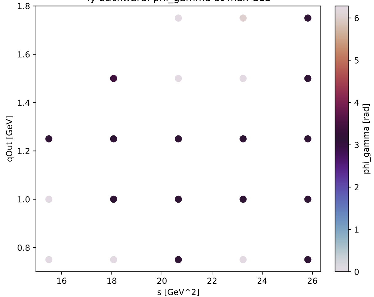
Ty backward: phi_gamma at max C13
