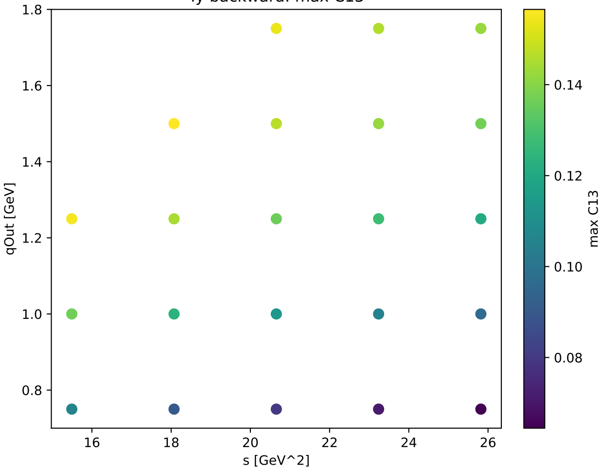
Ty backward: max C13
