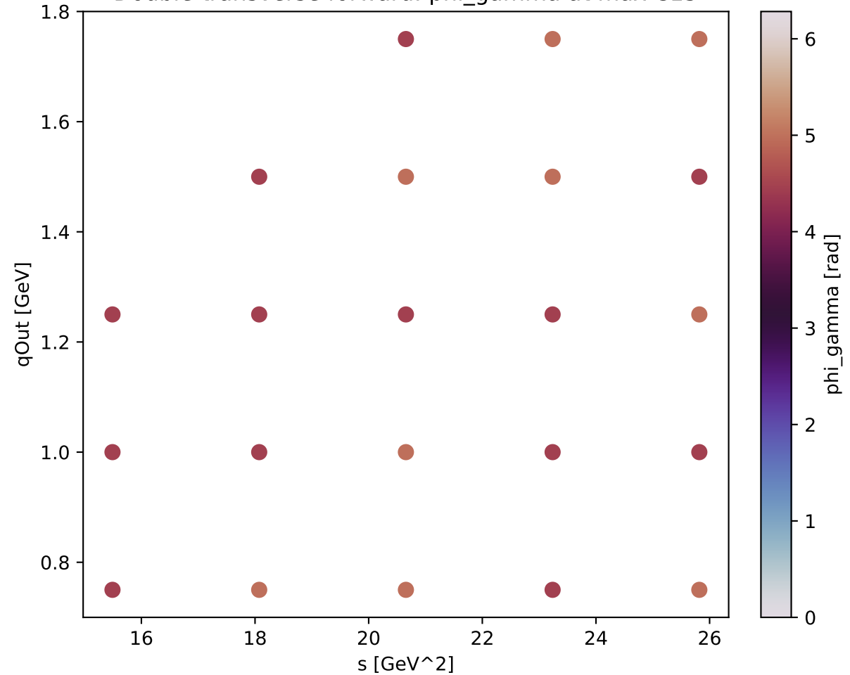
Double transverse forward: phi_gamma at max C13
