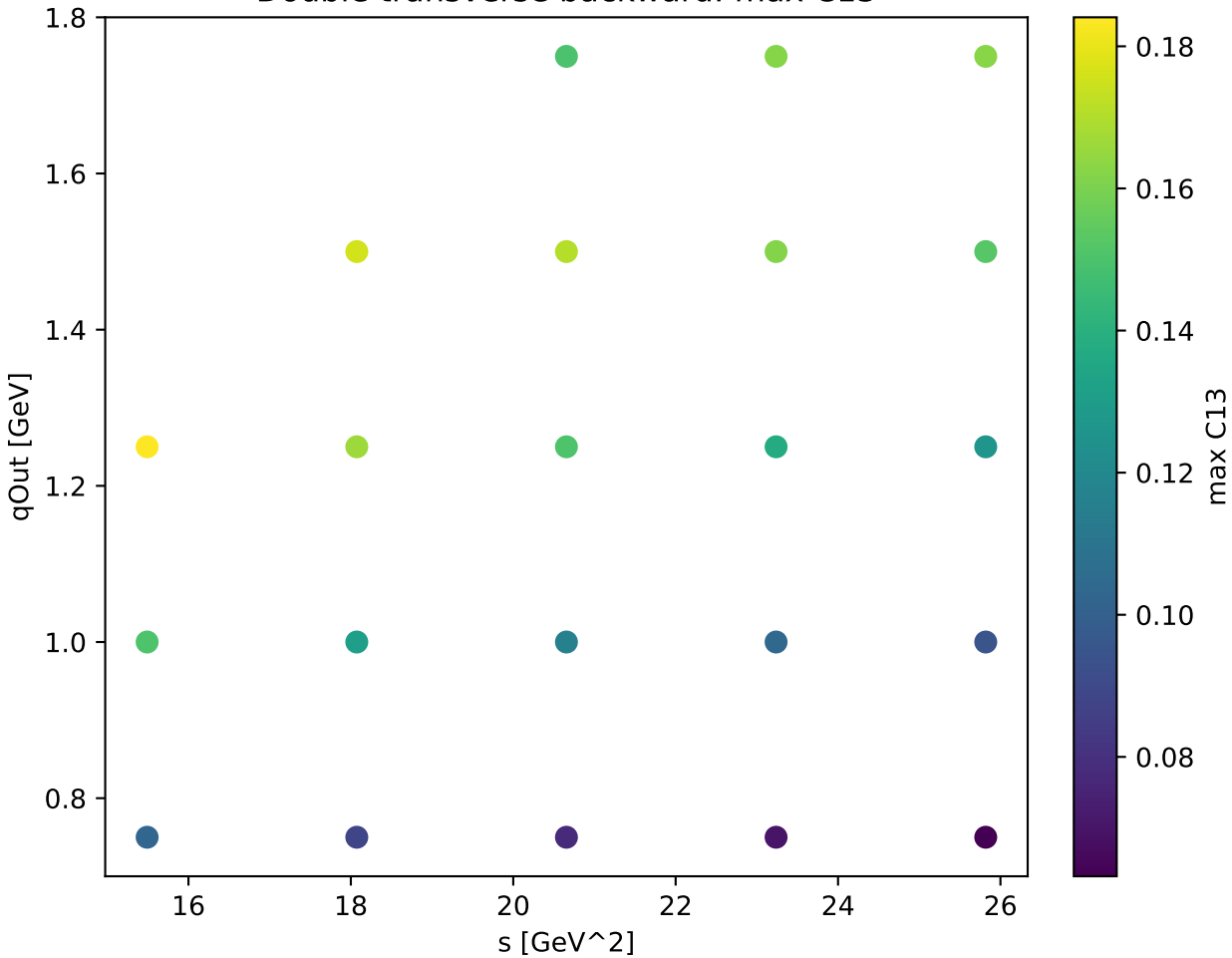
Double transverse backward: max C13
