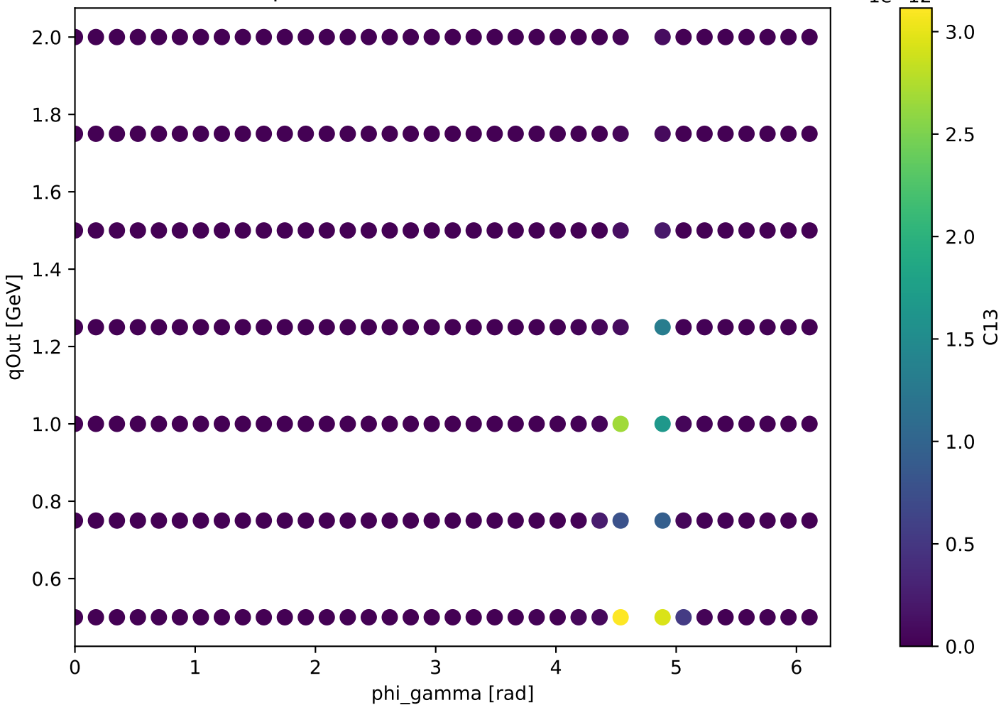
Unpolarized forward: C13 at s=25.64
