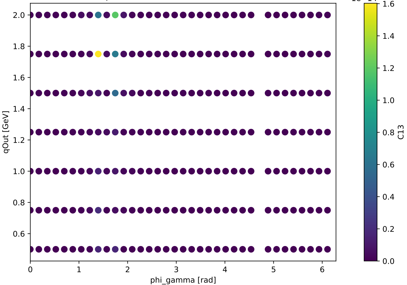
Unpolarized backward: C13 at s=27.97
