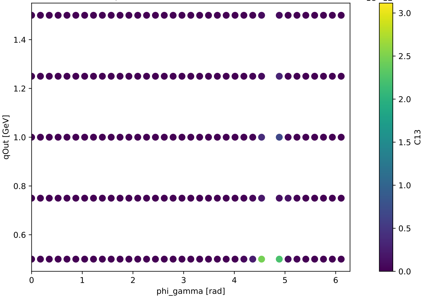
Unpolarized forward: C13 at s=16.32
