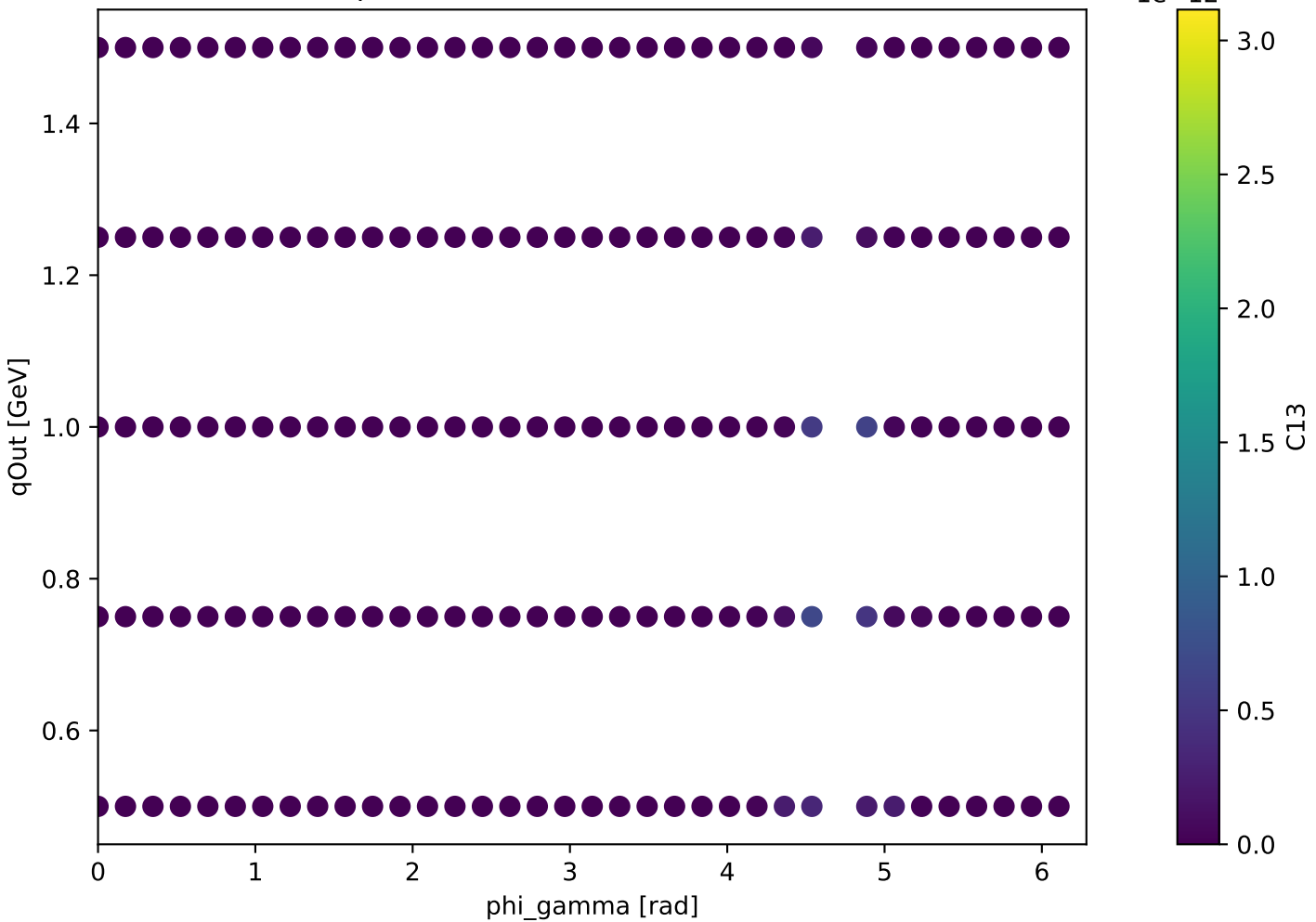
Unpolarized forward: C13 at s=18.65
