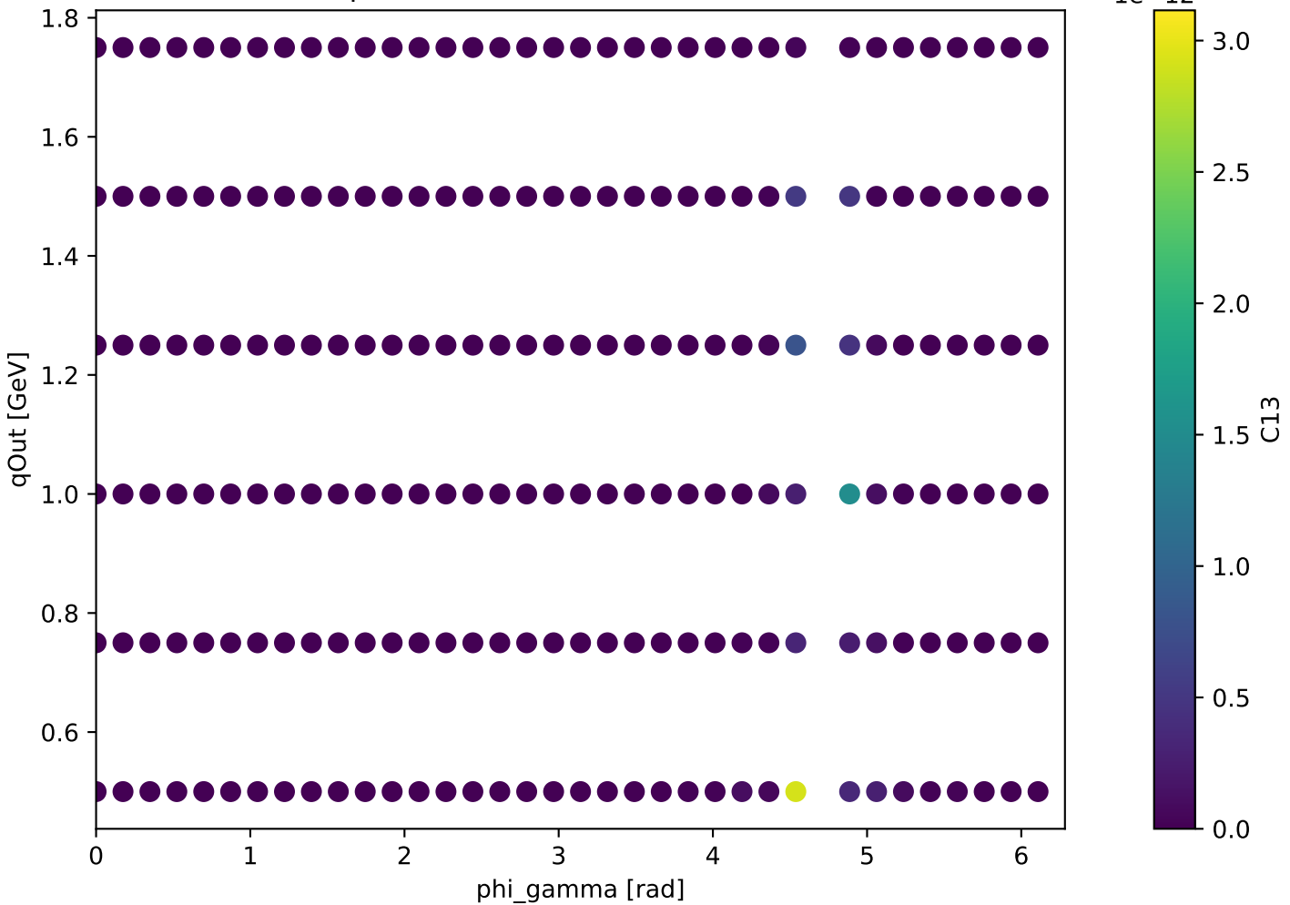
Unpolarized forward: C13 at s=23.31
