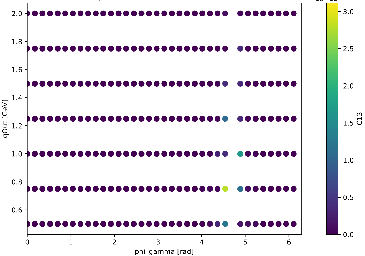
Unpolarized forward: C13 at s=27.97
