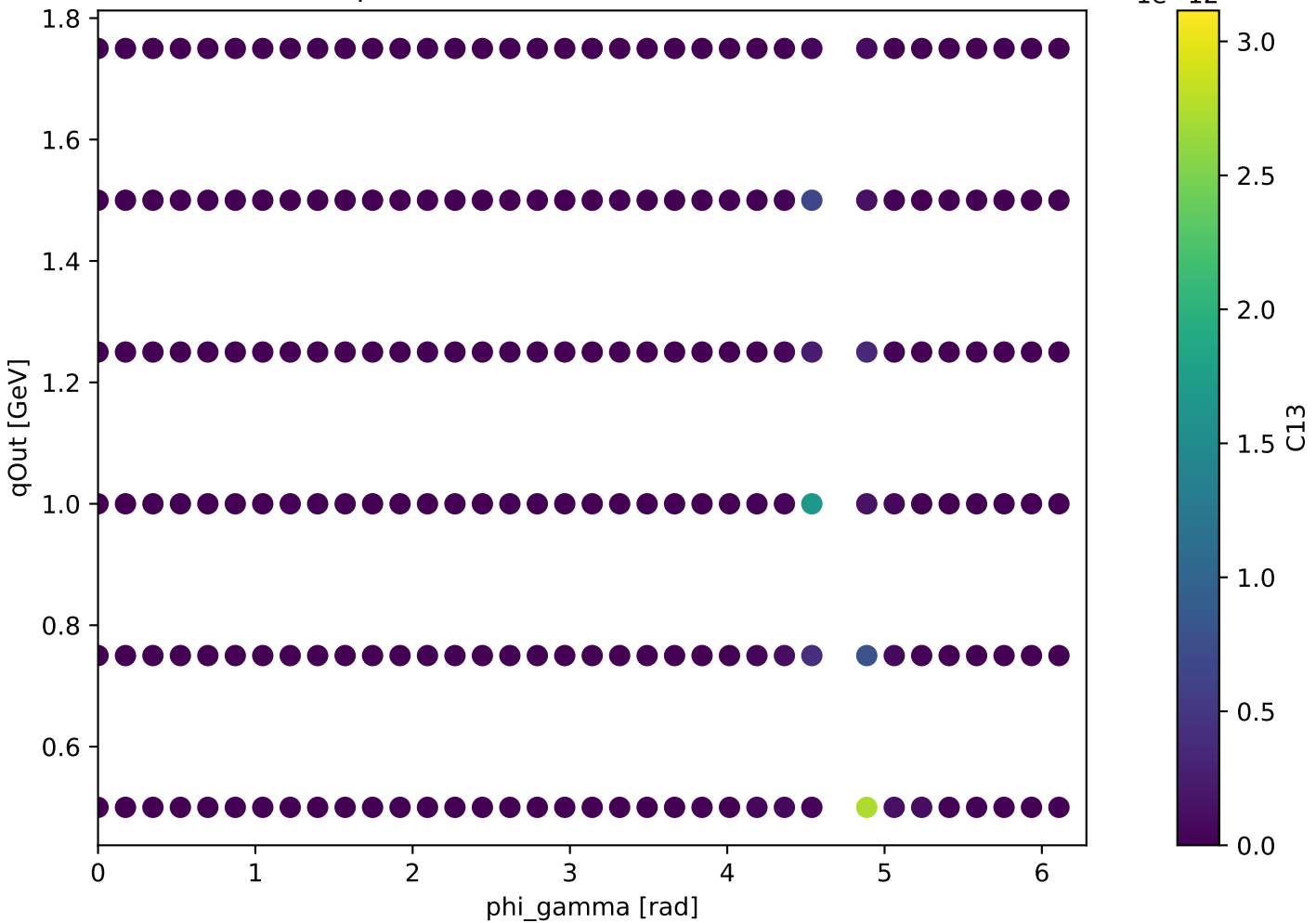
Unpolarized forward: C13 at s=20.98
