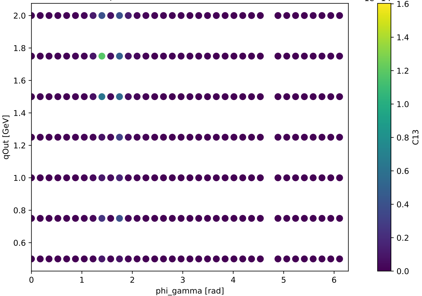
Unpolarized backward: C13 at s=25.64
