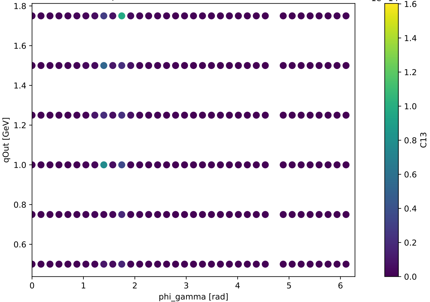
Unpolarized backward: C13 at s=20.98
