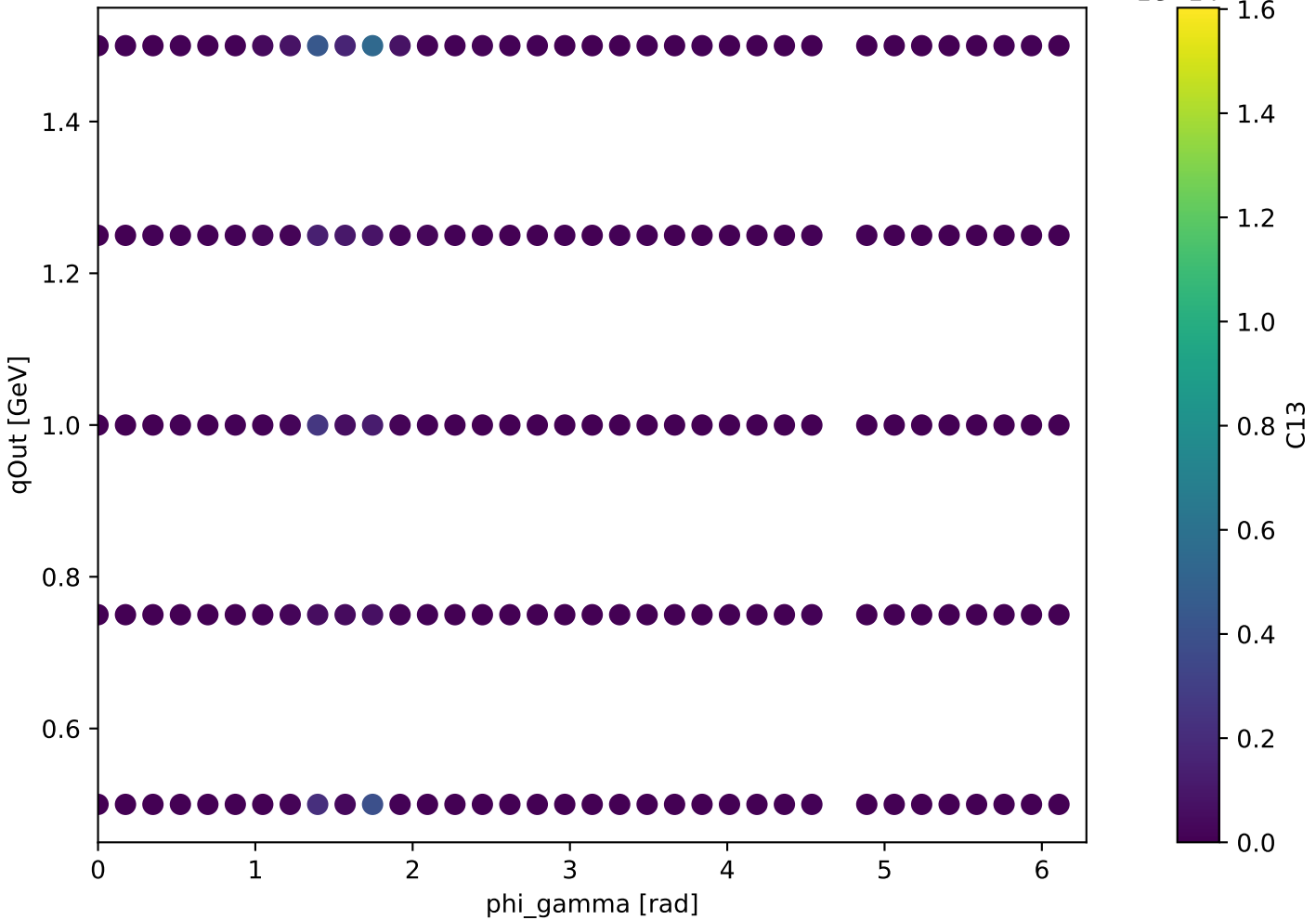
Unpolarized backward: C13 at s=18.65
