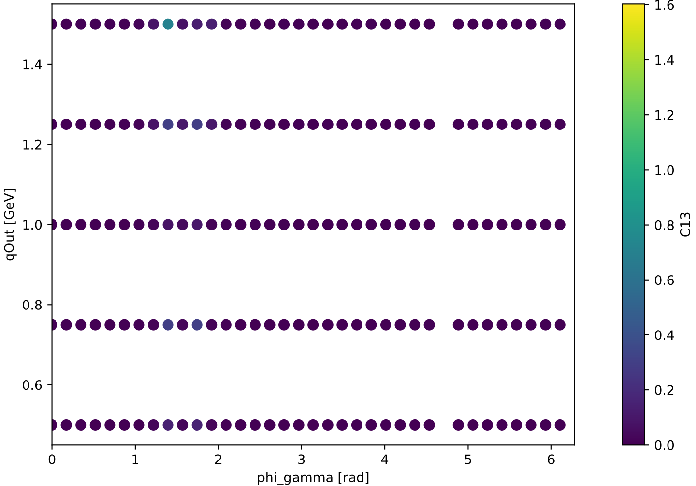
Unpolarized backward: C13 at s=16.32
