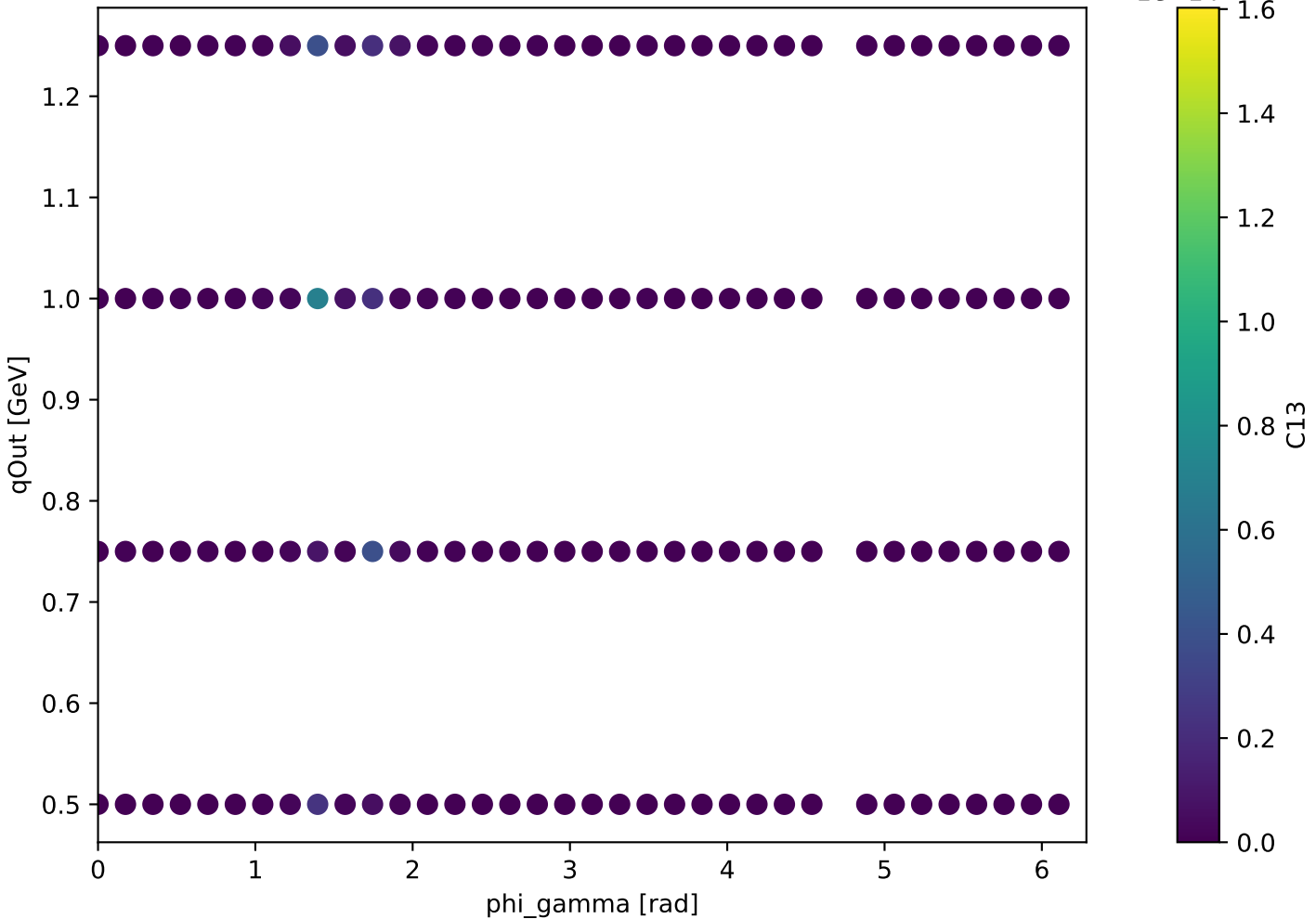
Unpolarized backward: C13 at s=13.99
