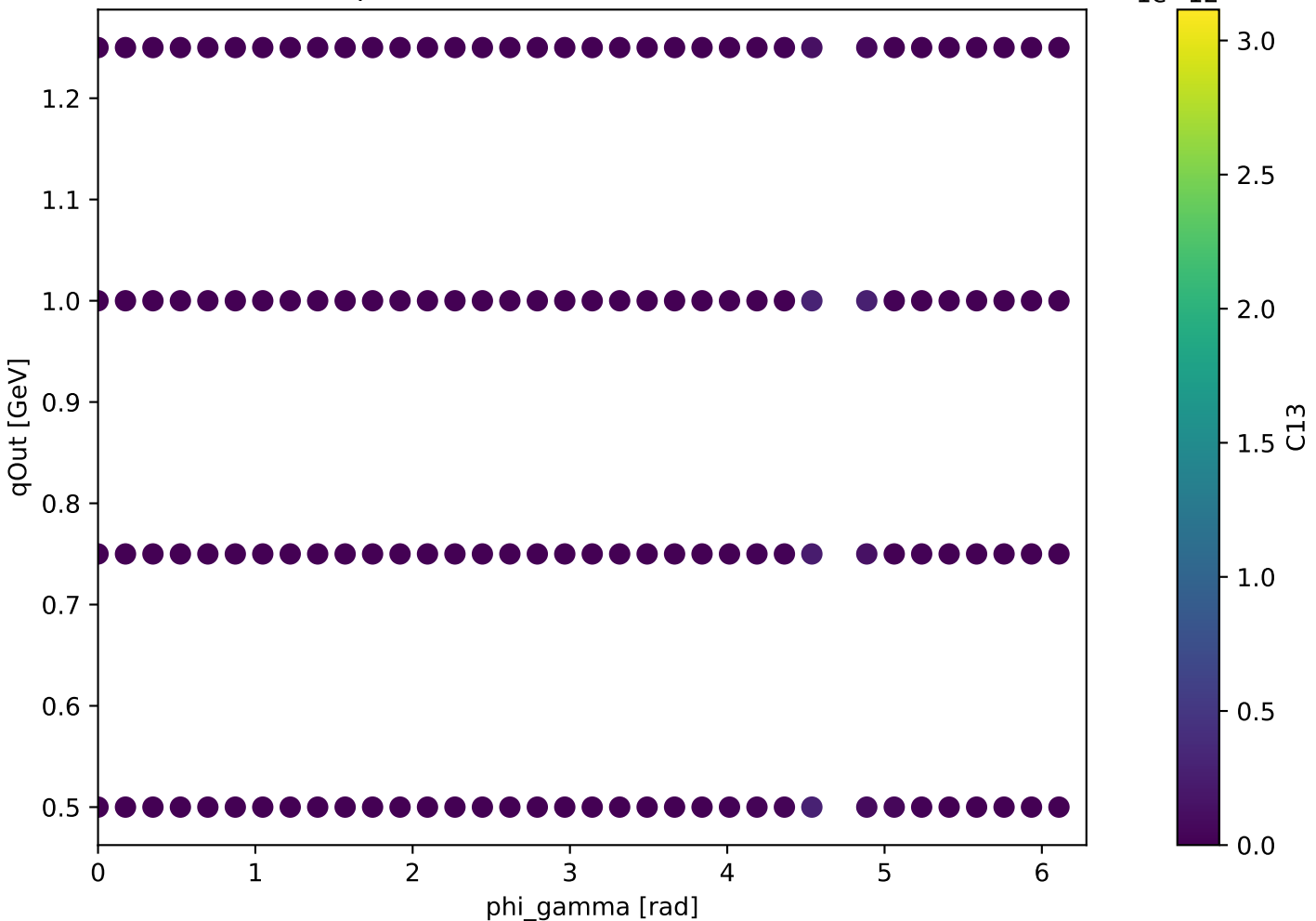
Unpolarized forward: C13 at s=13.99
