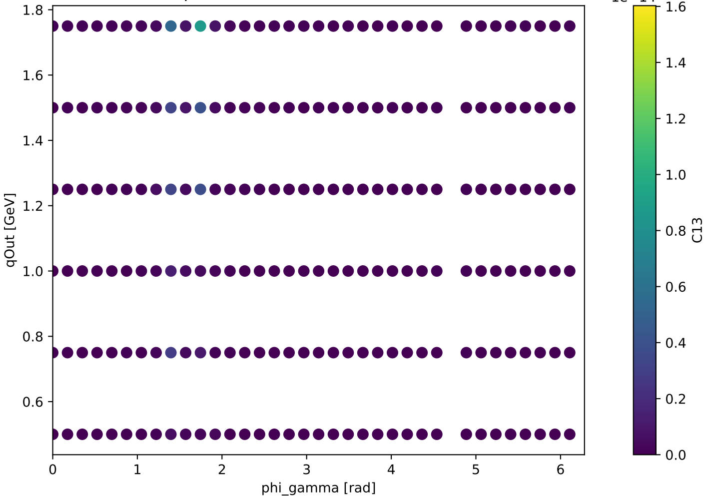
Unpolarized backward: C13 at s=23.31
