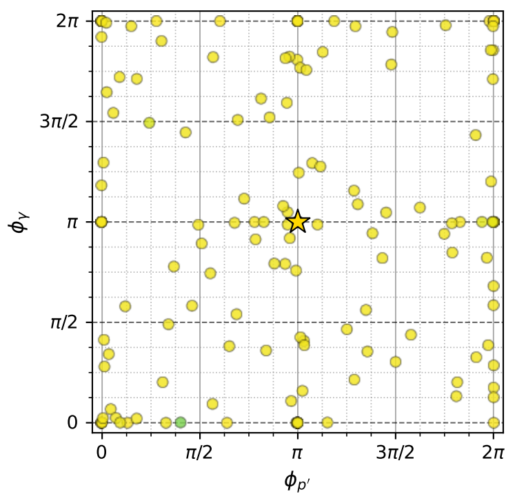
muon: polarization cluster P1 (contours omitted)
