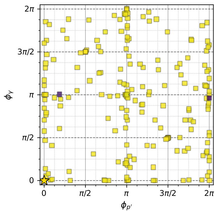
muon: polarization cluster P2 (contours omitted)
