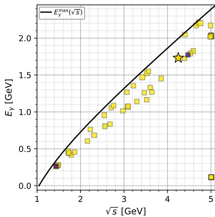
muon: polarization cluster P2 (contours omitted)
