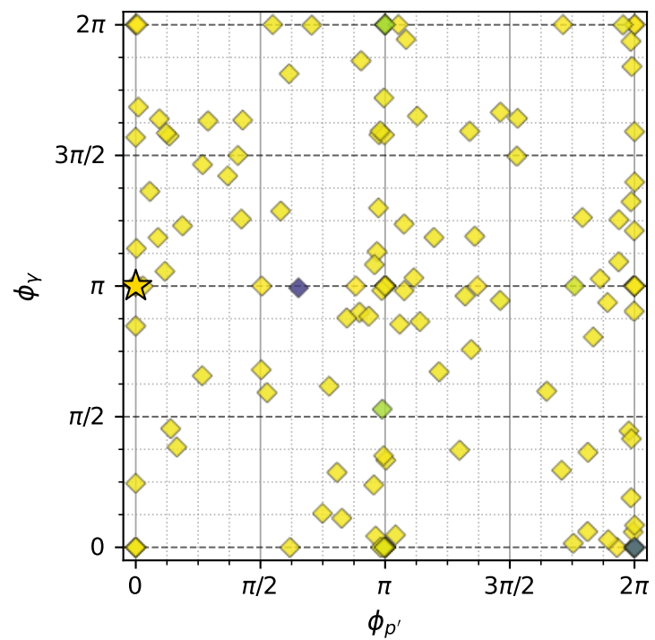
muon: polarization cluster P4 (contours omitted)
