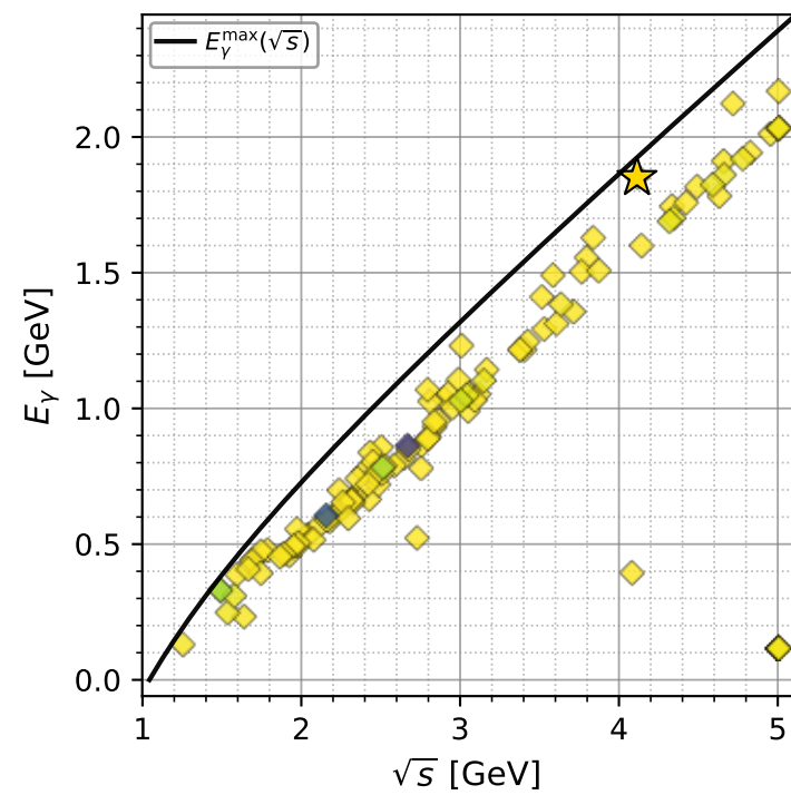
muon: polarization cluster P4 (contours omitted)
