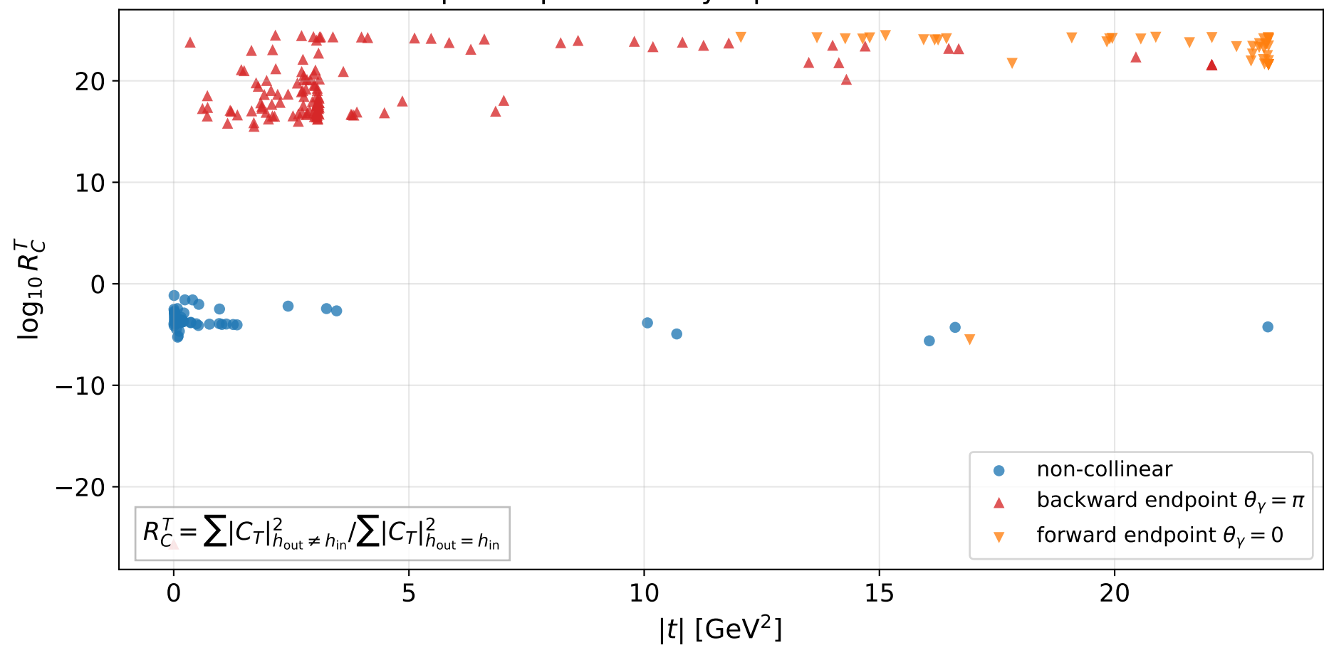
Compton lepton-helicity flip versus conservation
