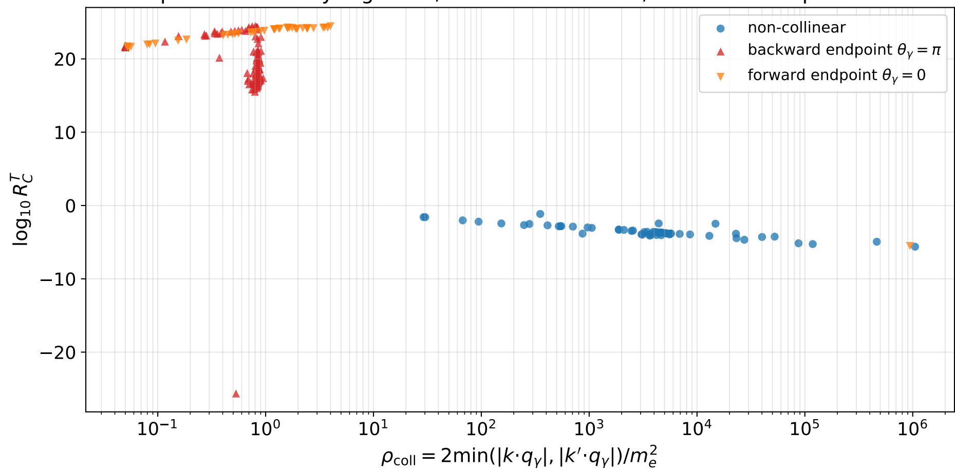
The endpoint-collinearity regulator, rather than t alone, controls the flip enhancement
