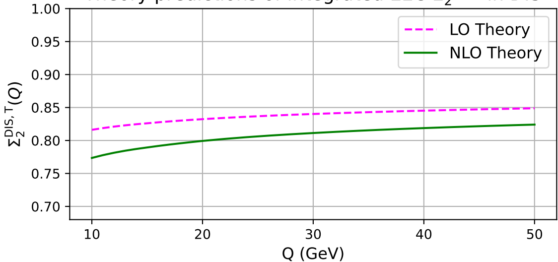
Theory predictions of integrated EEC \Sigma_2^{\text{DIS}, T} in DIS
