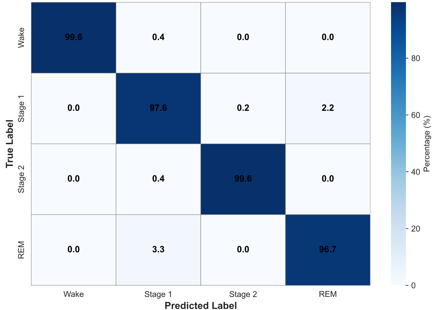
Confusion Matrix (Percentage)
